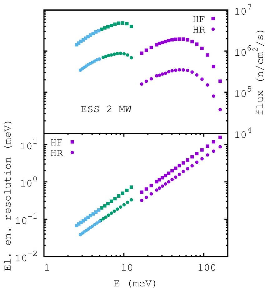
Fig. 32. Results of Vites simulations of T-REX for flux and elastic energy resolution are shown as a function of incident energy at 2 MW ESS source power, for two anticipated chopper configurations termed HF (highest flux) and HR (highest resolution).
