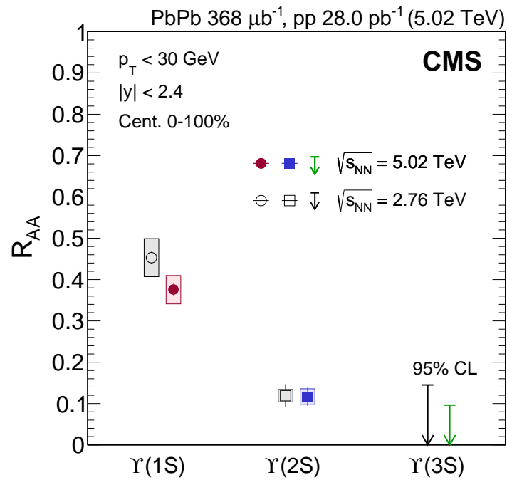
Figure 7: Comparison of R_{AA} values for the Y(1S) , Y(2S) and Y(3S) mesons at \sqrt{s_{NN}} = 5.02 \text{ TeV} and \sqrt{s_{NN}} = 2.76 \text{ TeV} [21] for integrated centrality in the full kinematic range. The error bars represent the statistical uncertainties and the boxes the systematic uncertainties, including global uncertainties.
