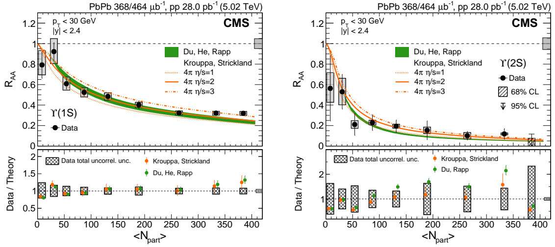
Figure 6: Nuclear modification factors for the \Upsilon(1S) (left) and \Upsilon(2S) (right) mesons as a function of \langle N_{\text{part}} \rangle compared to calculations from Krouppa and Strickland [9], and Du, He, and Rapp [12]. The box at the dashed line at unity represents the global uncertainty from the integrated luminosity in pp collisions, N_{\text{MB}} in PbPb collisions, and the total uncertainty in the pp yields. The data to theory ratios are shown in the bottom panels. For Ref. [9], the points correspond to the 4\pi\eta/s = 2 curve, while the error bars show the difference between this one and the other two \eta/s curves. For Ref. [12], the points and error bars correspond to the center and width of the published theory band, respectively.
