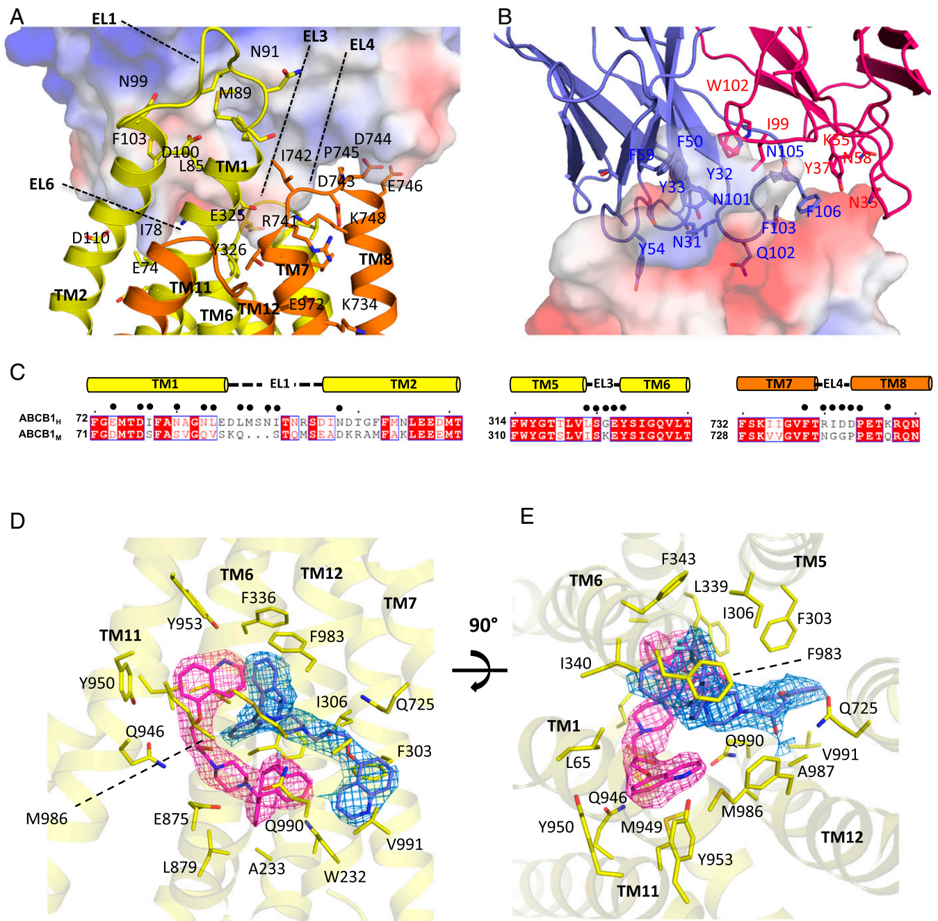
Fig. 2. Details of UIC2-binding interface and zosuquidar-binding pocket. (A) Close-up view of the ABCB1–UIC2 interface with the UIC2-Fab-binding region shown as an electrostatic surface potential map and ABCB1 shown in ribbon representation. TM helices and ELs of ABCB1 are labeled. ABCB1 residues interacting with UIC2-Fab or with a structural role in stabilizing the outward-closed conformation of ABCB1 are shown as sticks and labeled. (B) Similar view as in A, but with ABCB1 shown as semitransparent electrostatic surface potential map. UIC2-Fab is shown in ribbon representation and colored blue (heavy chain) or red (light chain). Select UIC2 residues within 5 Å of ABCB1 are shown as sticks. (C) Sequence alignments of EL1, EL3, and EL4 regions of ABCB1 H and mouse ABCB1, with secondary structure motifs shown above the sequences. Black dots represent residues of ABCB1 H within 4 Å of UIC2 as seen in our ABCB1 HM-X –UIC2 structure. (D) Ribbon diagram of ABCB1 viewed parallel to the membrane plane, with several TM helices removed for clarity. Two bound zosuquidar molecules are shown as pink and blue sticks, and the corresponding EM density is shown as pink and blue mesh. Selected ABCB1 residues within 4 Å distance of bound zosuquidar are shown as yellow sticks and labeled. (E) Similar to D but viewed from the external side of the membrane.
