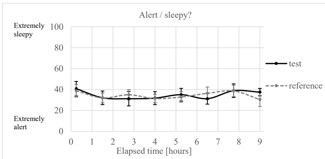
Figure 5. Average subjective alertness rating in the two conditions. Means across 6 participants ( \pm SEM) and 5 days per condition
