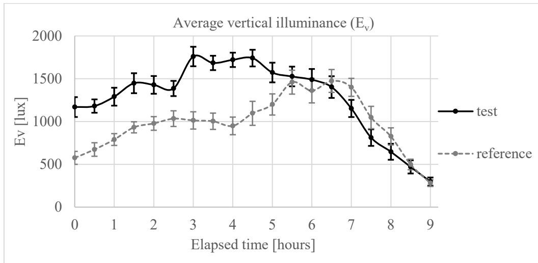
Figure 2. Average vertical illuminance at the eye level assessed by HDR vision sensors in the two conditions. Means across 6 participants ( \pm SEM) and 5 days per condition.
