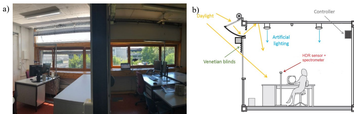
Figure 1. (a) View of the two office rooms. On the left side: test room, with ADS and automated control of venetian blinds and electric lighting; on the right side: reference room, with ADS closed and manual control of blind and lighting. (b) Cross-section scheme of an office room.
