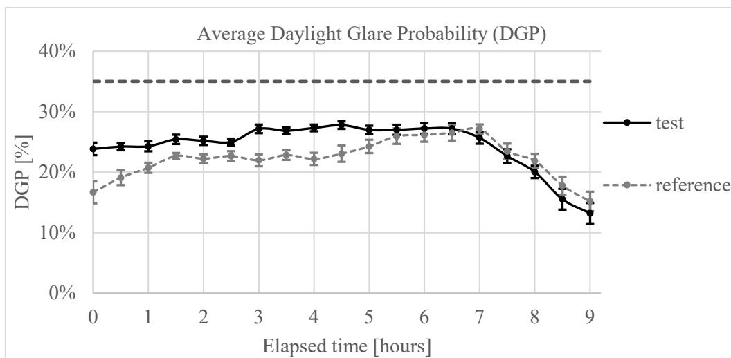
Figure 3. Average Daylight Glare Probability (DGP) assessed by HDR vision sensors in the two conditions. The thick dashed line indicates the threshold for perceptible glare sensation (lower is better). Means across 6 participants ( \pm SEM) and 5 days per condition.
