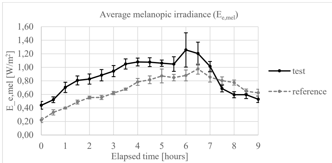
Figure 4. Average melanopic irradiance in the two conditions. Means across 6 participants ( \pm SEM) and 5 days per condition
