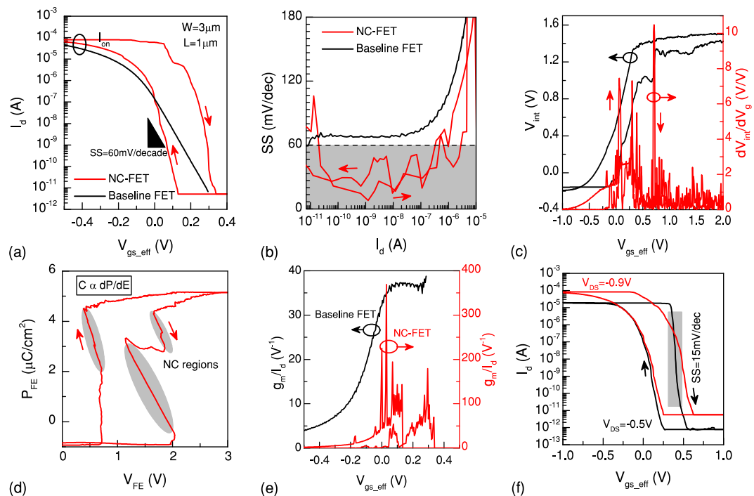
Figure 6. p-type NC-FET with a reduced hysteresis. (a) Input transfer characteristic of an NC-FET with a small hysteresis of 200 mV at |V_{ds}| = 900 mV. (b) A sub-thermal swing well below 60 mV/decade is obtained. (c) Measurement of the internal node shows a significant voltage gain, having a peak of 10 V/V. (d) Polarization characteristic of the ferroelectric capacitor shows an effective NC in both branches. Two discrete NC regions are observable in the reverse sweep of the gate voltage due to the polycrystallinity of the ferroelectric film. (e) g_m/I_d is considerably enhanced and reached a value of 400 V^{-1} . (f) shows the impact of the drain-to-source electric field on the steepness and hysteresis of the NC-FET.
