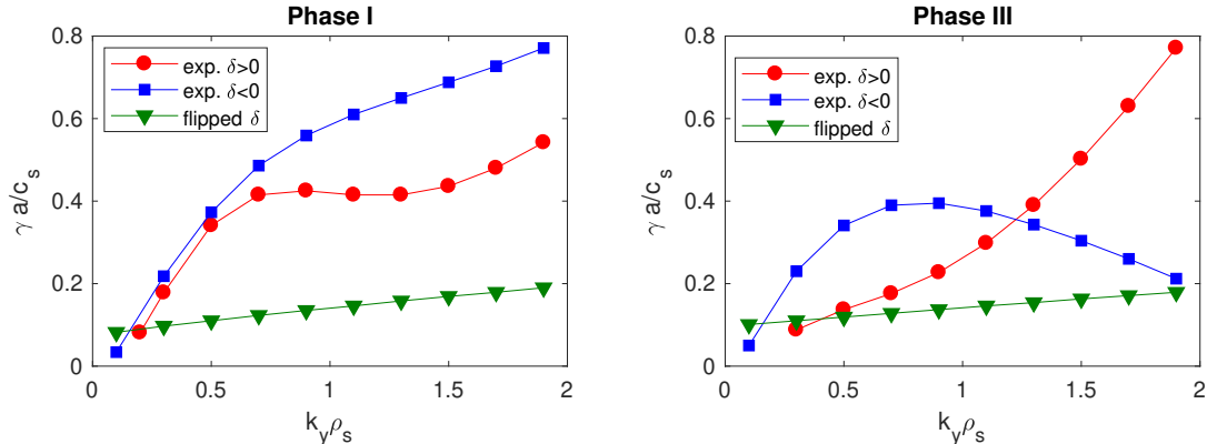
FIG. 5. Growth-rate \gamma as function of the toroidal mode number k_y \rho_s for (left) Phase I and (right) Phase III. Results for experimental condition corresponding to positive triangularity are shown with red circles, negative with blue squares and the ones obtained considering the equilibrium of \delta < 0 but profiles of \delta > 0 with green triangles.
