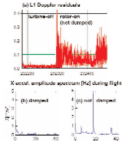
▲ FIGURE 4 Effect of vibrations on GPS and IMU sensors
