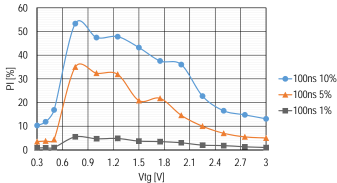
Fig. 5. Measured PI vs the TG control voltage at three different emulated PPG PI, 10%, 5% and 1%, for t_{transfer} of 100ns.
