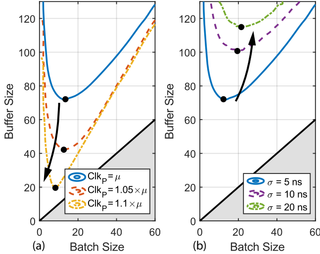
Fig. 6. Contour plots showing the optimal sizing of the RRAM-VAC circuit for (a) various f_P and (b) memory temporal variability.
