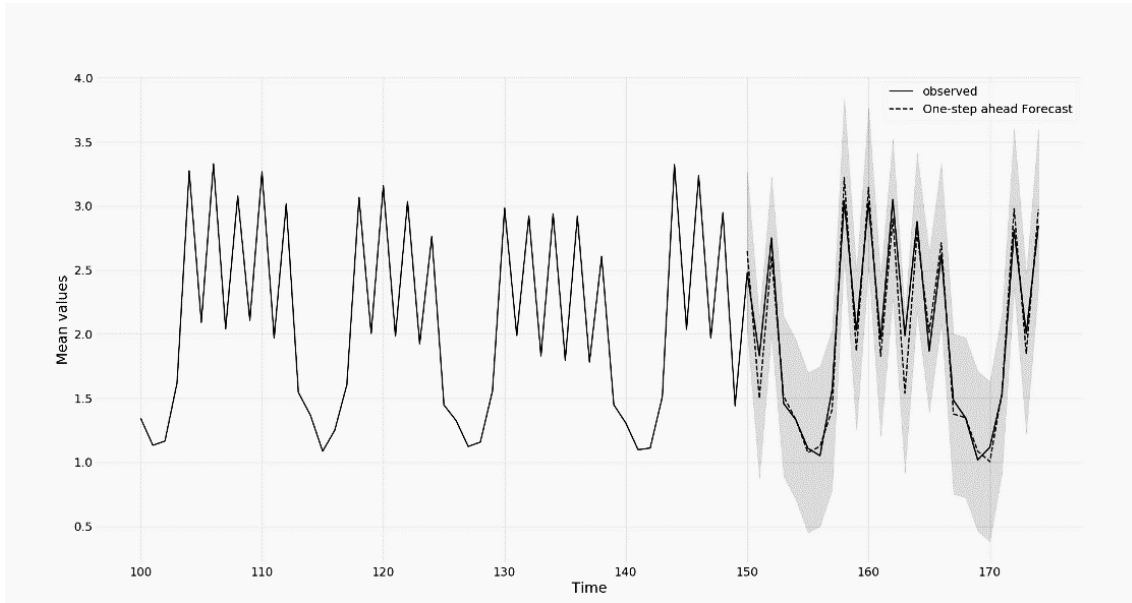
Figure 6. Model validation.
