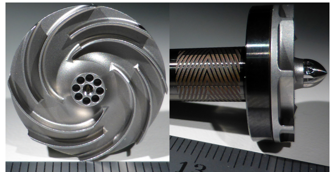
FIGURE 1. FRONT AND SIDE VIEW OF THE ANODE OFF-GAS RECIRCULATION FAN, ADAPTED FROM [6] (1 TICK = 1 MM).
