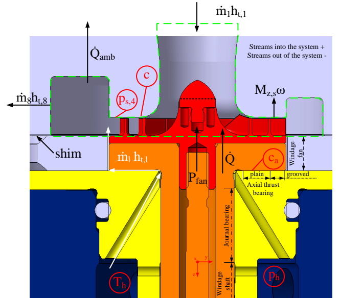
FIGURE 5. OVERVIEW OF ENTHALPY, POWER, AND HEAT INPUT, RESPECTIVELY OUTPUT TO THE FAN MEASUREMENT SYSTEM.
