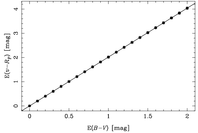
Figure A3. Comparison between the colour excesses measured in the (v - R_F) colour as a function of fictitious E(B - V) artificially introduced in the spectra of the reddening-free stellar subsample. Although we are using the same symbols as those used in Fig. A2, it is clear that the scatter introduced by distinct atmospheric stellar parameters is almost negligible. The relation is nicely fitted by a second-order polynomial.
