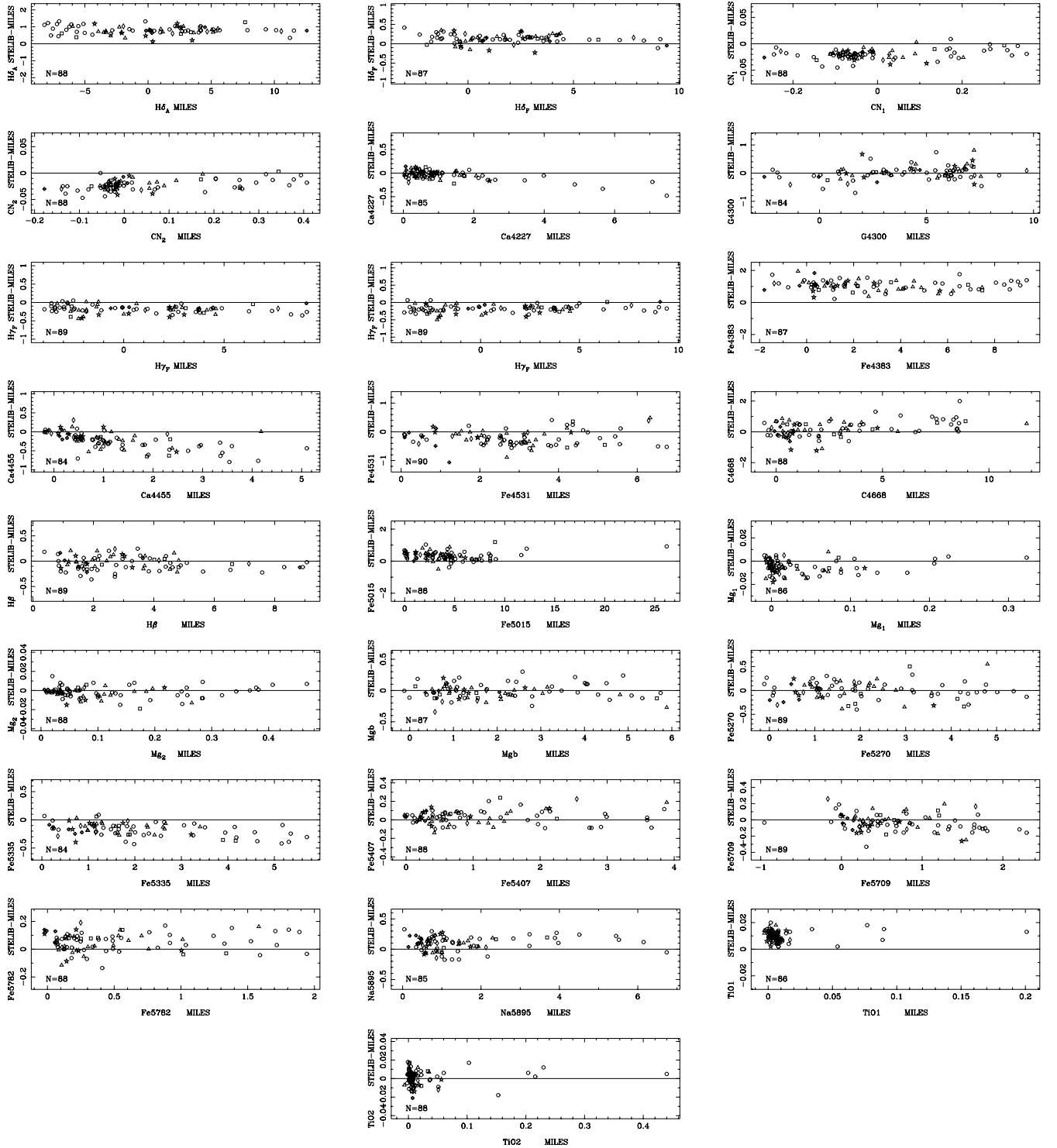
Figure 13. Differences between the Lick/IDS indices measured in MILES and STELIB spectra against MILES’ indices. In each panel, the number of stars in the comparison is indicated. Stars with different metallicities are displayed with different symbols as in Fig. 1.
