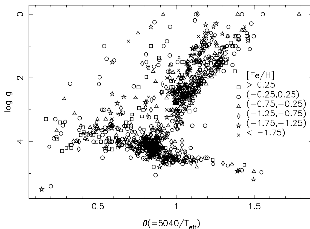
Figure 1. Gravity–temperature diagram for the library stars. Different symbols are used to indicate stars of different metallicities, as shown in the key.
