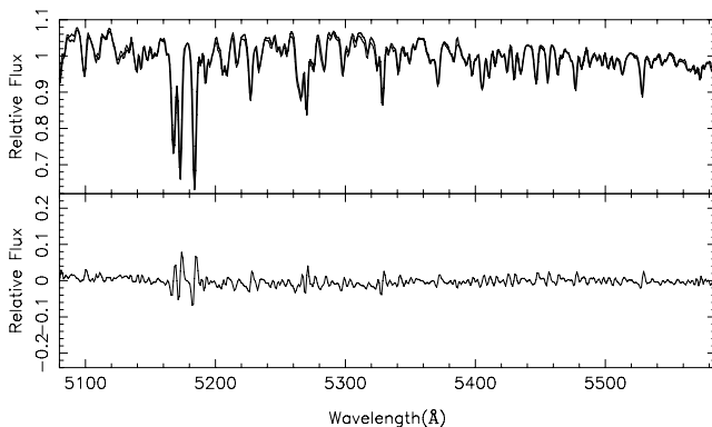
Figure 5. Red (thick line) and blue (thin line) spectra of the star HD 157214 in the spectral range in common between the two instrumental configurations.
