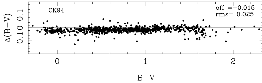
Figure 8. Residuals of the comparison of synthetic with empirical (B - V) colours from the Lausanne data base. The numbers within the panels show the derived mean offsets and standard deviations. See the text for details.
