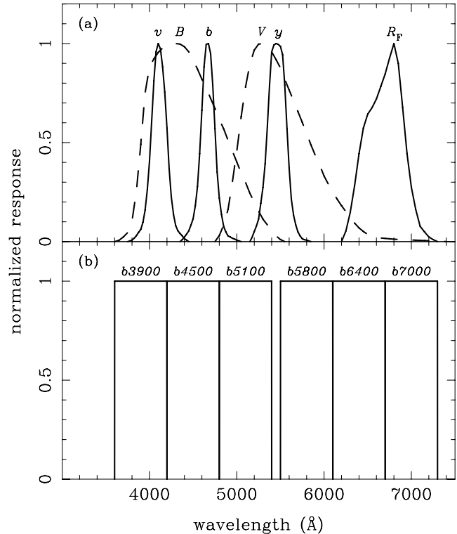
Figure A1. Normalized response functions of typical filters – panel (a) – and special filters – panel (b) – employed to estimate colour excesses in the subset of stellar spectra without published reddenings. The displayed filters are the Johnson’s B and V , the Strömgren’s v , b and y , the Couch–Newell’s R_F , and box functions of 600-Å width centred at 3900, 4500, 5100, 5800, 6400 and 7000 Å.
