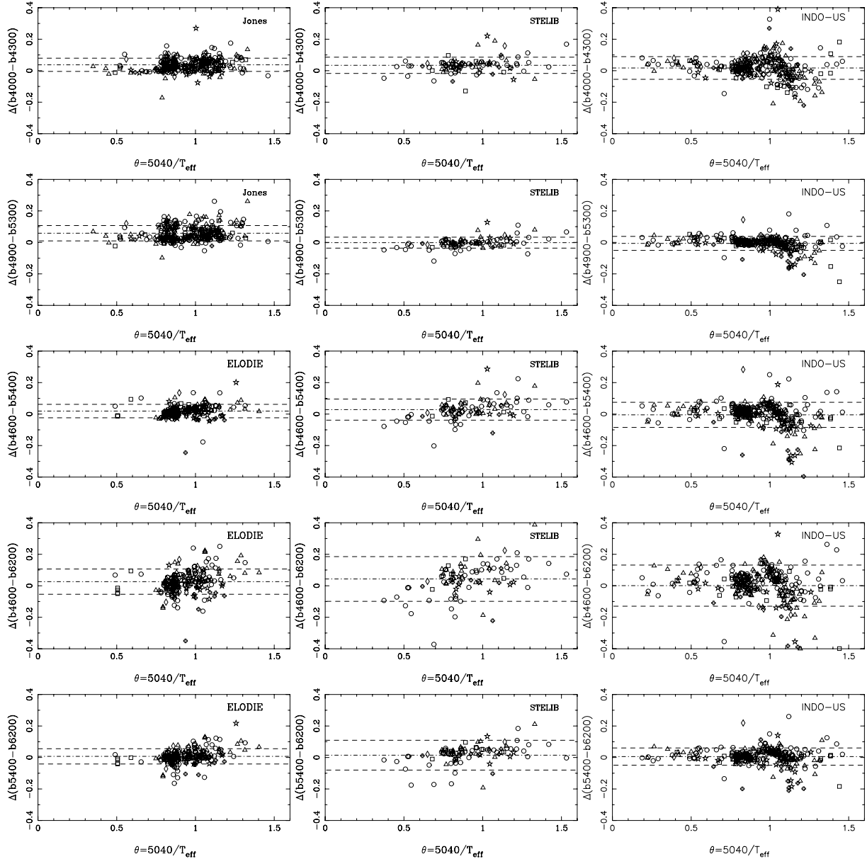
Figure 9. Residuals of the comparison of synthetic colours measured in MILES with those measured in other stellar libraries, versus \theta = 5040/T_{\text{eff}} . The different symbols indicate stars of different metallicities, as coded in Fig. 1. The dashed lines correspond to 1\sigma rms.
