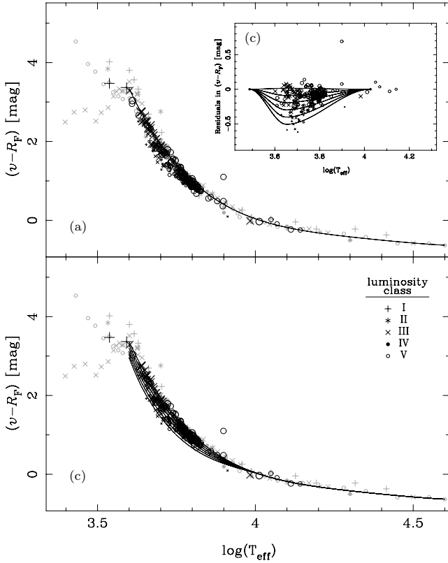
Figure A2. Variation of the (v - R_F) colour as a function of effective temperature. The different symbols correspond to distinct luminosity classes, as explained in the key, whereas the symbol sizes are indicative of metallicity (larger symbols for higher [\text{Fe}/\text{H}] ). In panels (a) and (c), we have overplotted, with light-grey symbols, the stellar sample of Pickles (1998). The inclusion of the latter has allowed us to obtain an initial fit only dependent on T_{\text{eff}} up to the highest temperature side. The inset in panel (b) corresponds to a zoom in the intermediate temperature interval (after subtracting the initial fit), where the dependence on metallicity is more important. A new set of polynomials were fitted in this interval to reproduce the behaviour in both T_{\text{eff}} and [\text{Fe}/\text{H}] (where metallicities are [\text{Fe}/\text{H}] = -2.0, -1.5, -1.0, -0.5, 0.0 and +0.5 from bottom to top panel). The combination of these polynomials and the initial fit leads to the final fitting functions displayed in panel (c). Note that these functions are not extrapolated below \log(T_{\text{eff}}) < 3.6 .
