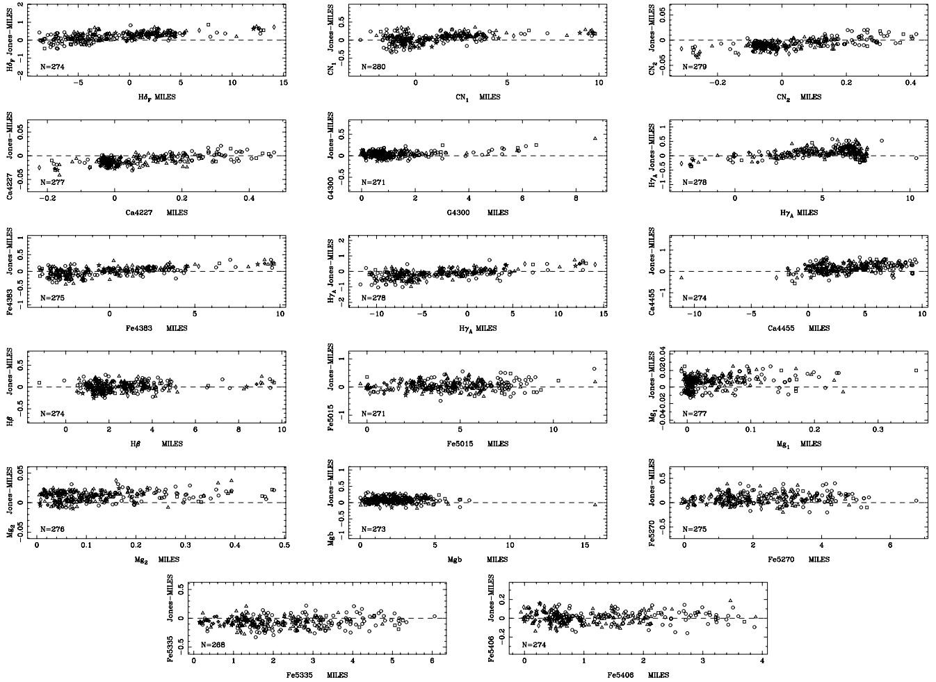
Figure 12. Differences of the Lick/IDS indices between MILES spectra and Jones’ library against the indices measured in MILES. The number of stars in the comparison is displayed within each panel. The meaning of the symbols is the same as in Fig. 1.
