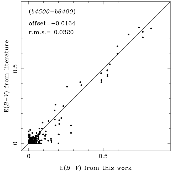
Figure A4. Comparison of E(B - V) values from the literature with E(B - V) estimations obtained from the excesses measured in the (b4500 - b6400) colour, following the method described in Appendix A.
