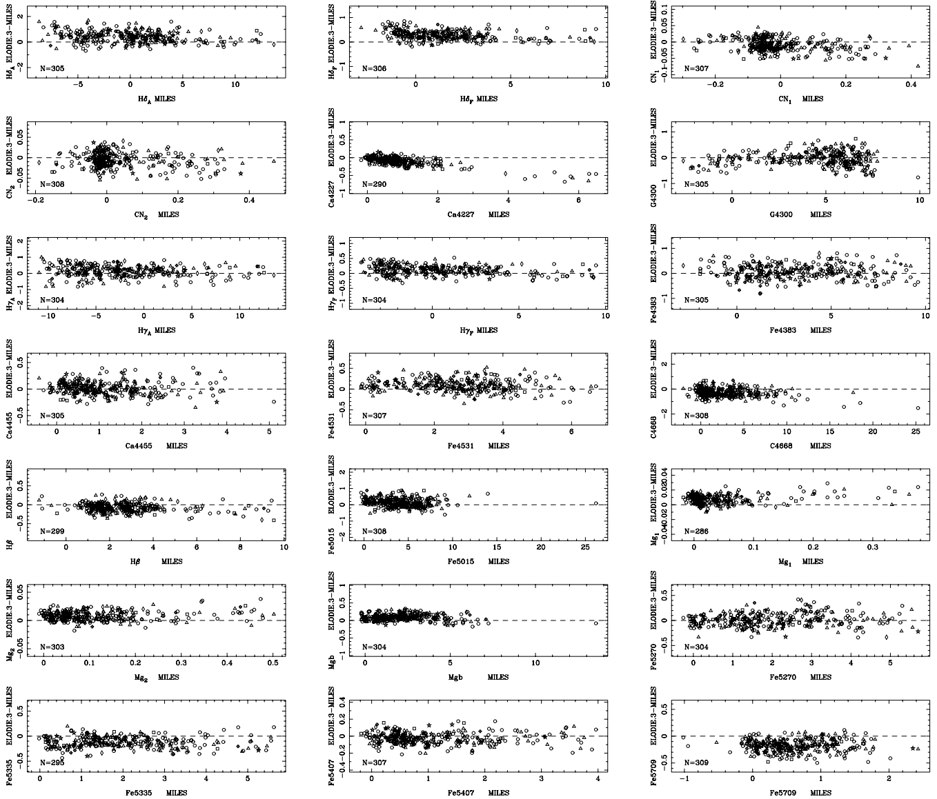
Figure 14. Differences between the Lick indices measured on MILES and in the most recent version of ELODIE spectra against MILES’ indices. In each panel, the number of stars fitted and the slope of the fit are indicated. Stars with different metallicities are displayed with different symbols as in Fig. 1.
