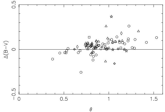
Figure 11. Residuals of the comparison of synthetic (B - V) colours from the STELIB data set with those from MILES [ \Delta(B - V) = (B - V)_{\text{STELIB}} - (B - V)_{\text{MILES}} ]. The symbols are the same as in Fig. 1.
