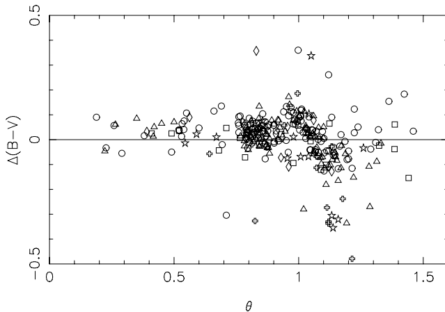
Figure 10. Residuals of the comparison of synthetic (B - V) colours from the INDO-US library with those from MILES [ \Delta(B - V) = (B - V)_{\text{INDO-US}} - (B - V)_{\text{MILES}} ]. The symbols are the same as in Fig. 1.
