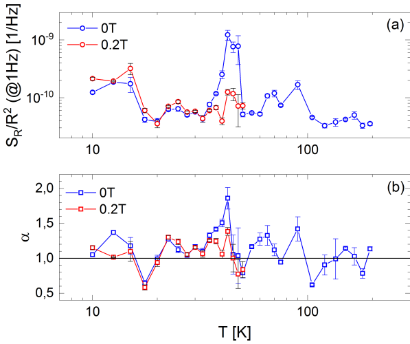
Fig. 2. (a) Normalized resistance noise PSD S_R/R^2 ( f = 1\text{ Hz} ) against temperature T for different magnetic fields B = 0\text{ T} and B = 0.2\text{ T} . (b) Frequency exponent \alpha against temperature T at for different magnetic fields, namely B = 0\text{ T} and B = 0.2\text{ T} . The horizontal line marks \alpha = 1 , see text for details.
