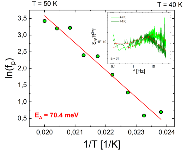
Fig. 3. Arrhenius plot of the corner frequency f_c of the Lorentzian contributions against 1/T . A linear fit yields the activation energy E_A = 70\text{ meV} of the underlying two-level-process. Inset: Selected spectra at T = 44\text{ K} and 47\text{ K} in a plot S_R/R^2 \times f vs. f with corresponding Lorentzian fits.
