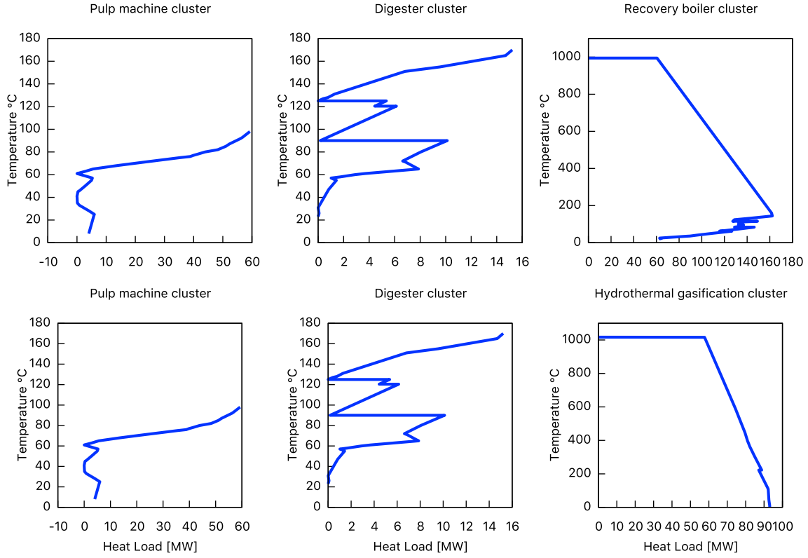
Figure 3: Grand composite curve of MER of conventional Kraft mill and hydrothermal gasification
