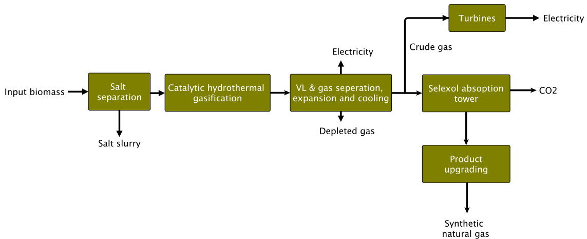
Figure 2: Block flow diagram of the catalytic hydrothermal gasification model, adapted from [15]
