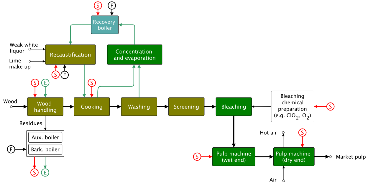
Figure 1: Block flow diagram of a generic Kraft process, adapted from [14]
