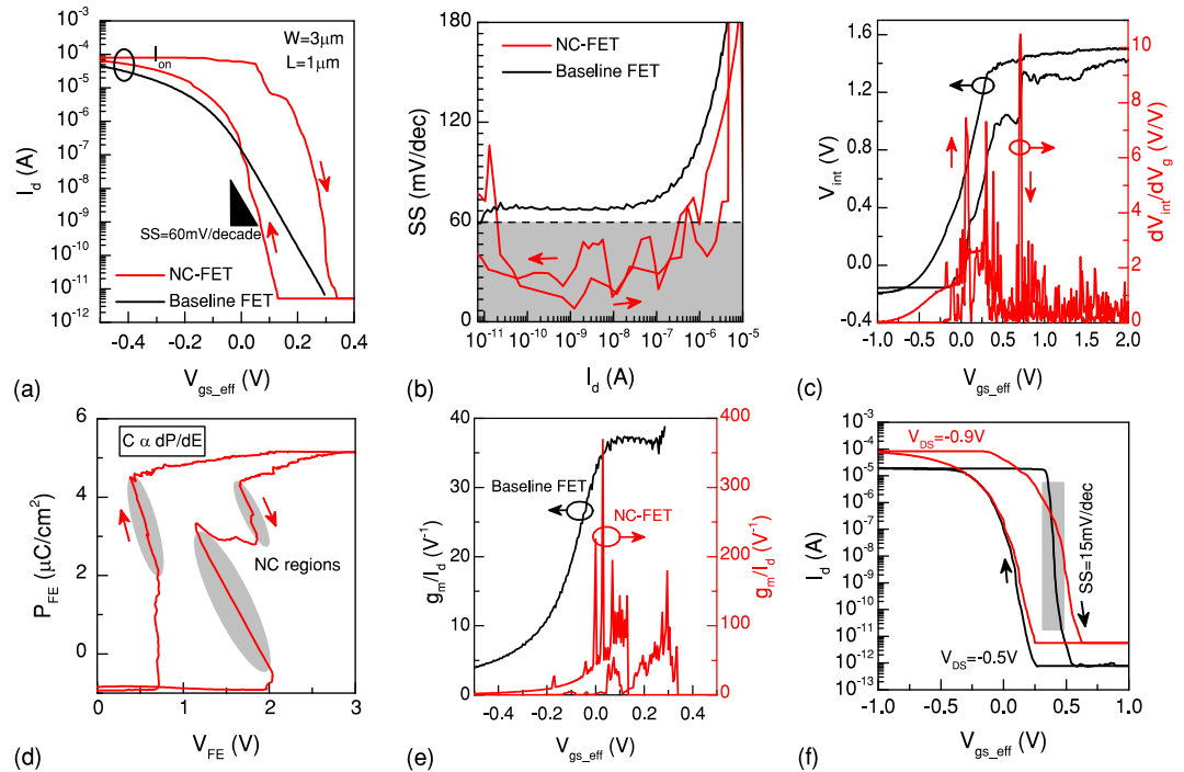
Figure 6. p-type NC-FET with a reduced hysteresis. (a) Input transfer characteristic of an NC-FET with a small hysteresis of 200 mV at |V_{ds}| = 900 mV. (b) A sub-threshold swing well below 60 mV/decade is obtained. (c) Measurement of the internal node shows a significant voltage gain, having a peak of 10 V/V. (d) Polarization characteristic of the ferroelectric capacitor shows an effective NC in both branches. Two discrete NC regions are observable in the reverse sweep of the gate voltage due to the polycrystallinity of the ferroelectric film. (e) g_m/I_d is considerably enhanced and reached a value of 400 \text{ V}^{-1} . (f) shows the impact of the drain-to-source electric field on the steepness and hysteresis of the NC-FET.
