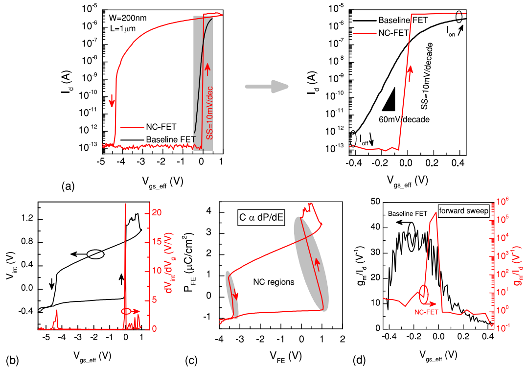
Figure 3. Hysteretic n-type NC-FET. (a) Transfer characteristic shows a super steep transition of 10 mV/decade together with a hysteresis of 4.5 V ( V_{ds} = 100 mV). (b) A remarkable amplification (defined as dV_{int}/dV_g ) up to 20 V/V is achieved in the regions corresponding to the negative slope of the polarization (c). Extracted current efficiency factor of the device represents a significant boosting, up to 10^5 V -1 (d).
