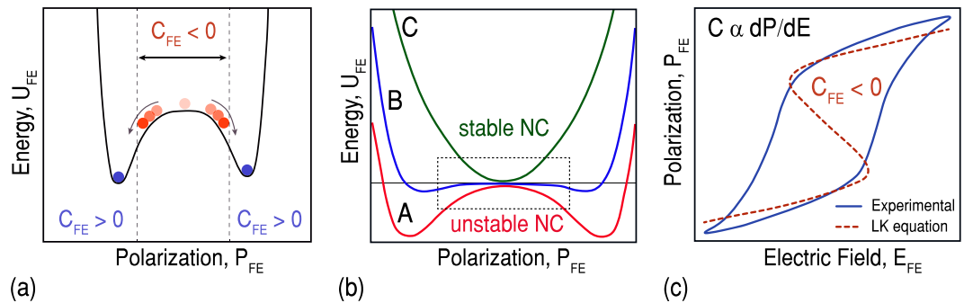
Figure 1. Negative capacitance in ferroelectric materials. (a) Energy density function of a ferroelectric capacitor in equilibrium, showing an effective NC while switching from one stable polarization state to the other one. (b) Ferroelectric's NC is unstable by itself (A), but it can be partially (B) or fully stabilized (C) by placing in-series with a positive capacitor. (c) Measured polarization vs. electric field of a PZT film (experimental) and the fitting results of LK equation (dashed curve).
