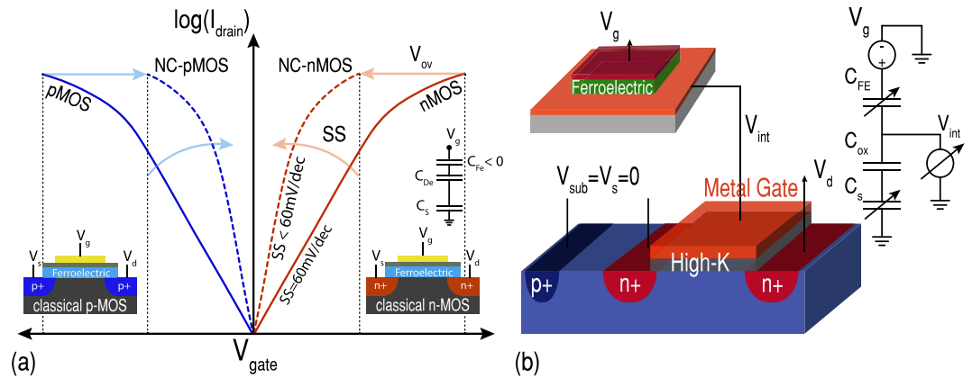
Figure 2. Negative capacitance MOSFET. (a) Performance boosting that can be achieved in both n- and p-type MOS transistors using NC of ferroelectrics in terms of SS reduction and overdrive improvement. (b) The employed experimental configuration of an n-type NC-FET including the capacitance model.
