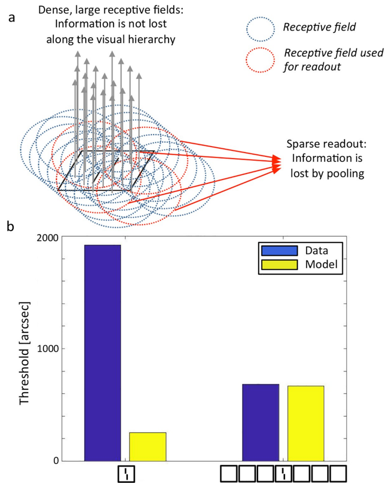
Fig 12. Hierarchical Sparse Selection model. a. The model posits that receptive fields along the visual hierarchy are large and dense. This allows for “lossless” transmission of information through the visual system. For instance, the offset of the vernier in this illustration is not corrupted by pooling thanks to the density of the receptive fields (blue and red circles). Crowding occurs because, when we try to access information, only a few sparse receptive fields are used for readout (red circles). Hence, crowding occurs at readout because of sparse sampling of receptive fields. This sparse readout can occur at any stage of visual processing, from low-level features (shown here) to faces. b. Uncrowding does not occur in the Hierarchical Sparse Selection model because performance is worse for the model on the 7 squares than the 1 square condition, contrary to human performance. NB. This model only produces a scalar output, there is no output image.
