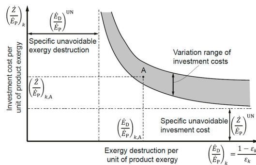
Figure 3. Definition of specific unavoidable exergy destruction (\dot{E}_D/\dot{E}_P)_k^{UN} and specific unavoidable investment cost (\dot{Z}/\dot{E}_P)_k^{UN} based on the expected relationship between investment cost and exergy destruction (or exergetic efficiency) for the k th component. (Reproduced from [86]).
