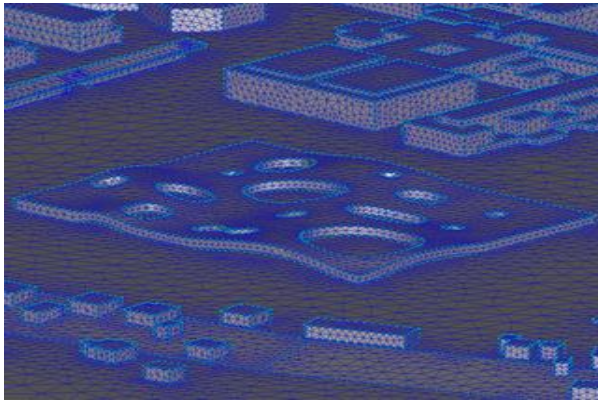
Figure 10. Autodesk CFD. Meshed model made by the Mesheres sizing command .
