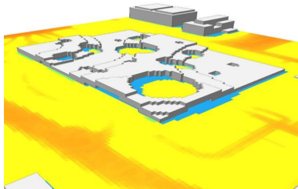
Figure 6. ENVI-met. MRT Output.
