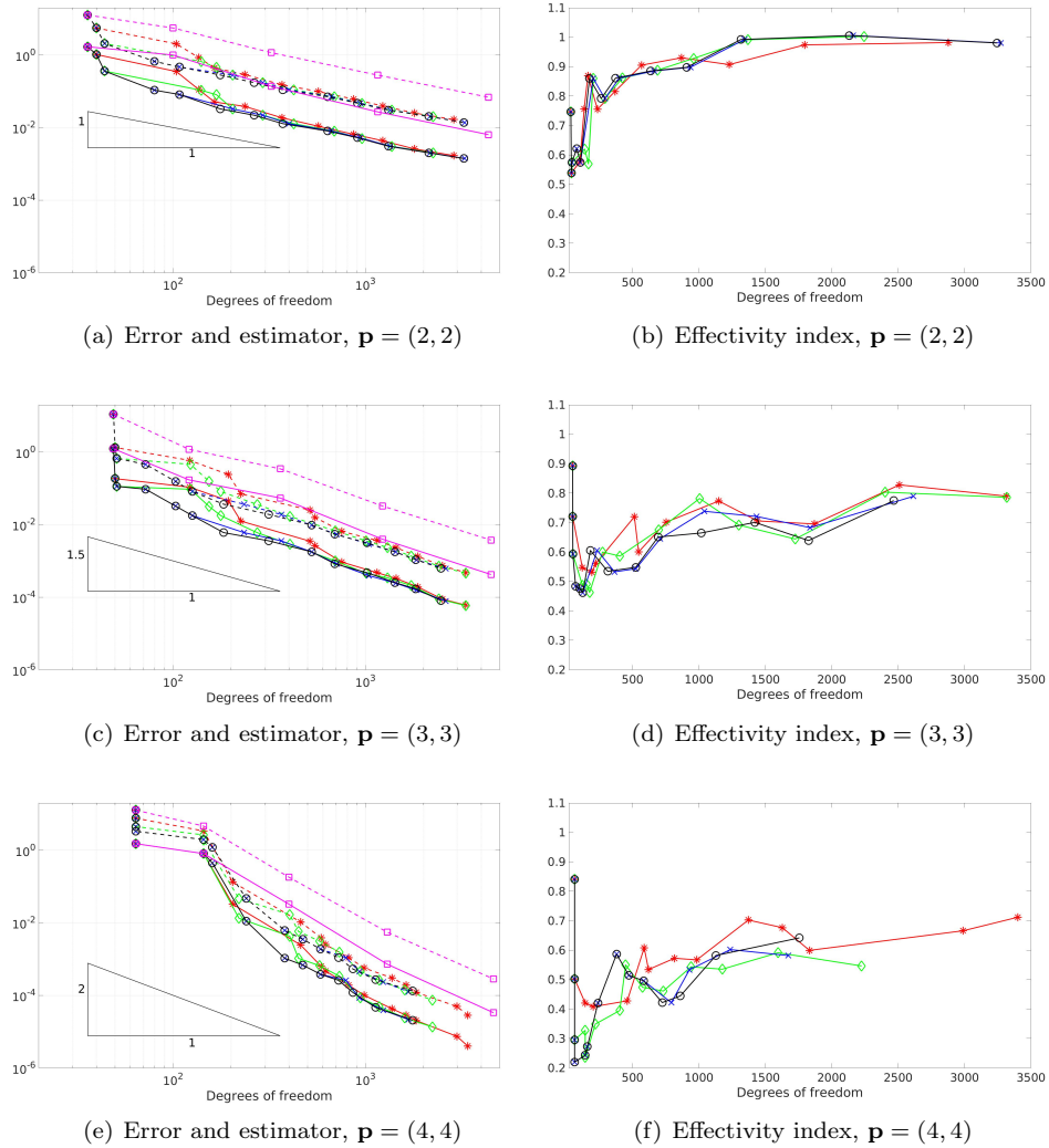
FIGURE 4. Numerical error and estimator (left) and effectivity index (right) for the smooth function with a peak. On the left, the error (solid lines) and the estimator (dashed lines) are plotted for different degrees. The red, green, blue and black lines (star, diamond, cross and circle markers, respectively) represent admissibility classes m = 2, 3, 4, \infty , respectively, while the magenta line (square marker) corresponds to uniform refinement. The same coloring and marking is used for the effectivity index (divided by 10) on the right figure.
