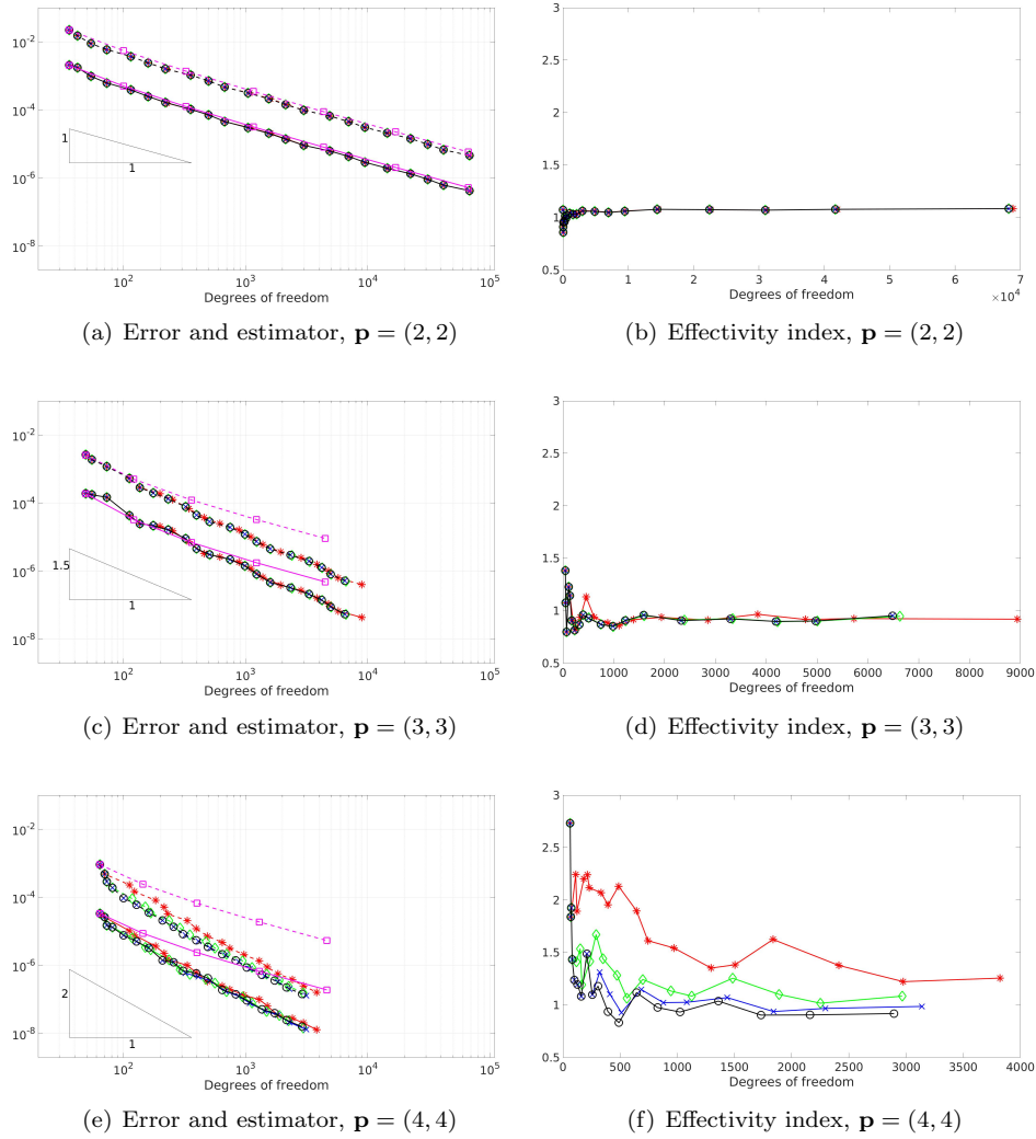
FIGURE 6. Numerical error and estimator (left) and effectivity index (right) for the example with singular solution. On the left, the error (solid lines) and the estimator (dashed lines) are plotted for different degrees. The red, green, blue and black lines (star, diamond, cross and circle markers, respectively) represent admissibility classes m = 2, 3, 4, \infty , respectively, while the magenta line (square marker) corresponds to uniform refinement. The same coloring and marking is used for the effectivity index (divided by 10) on the right figure.
