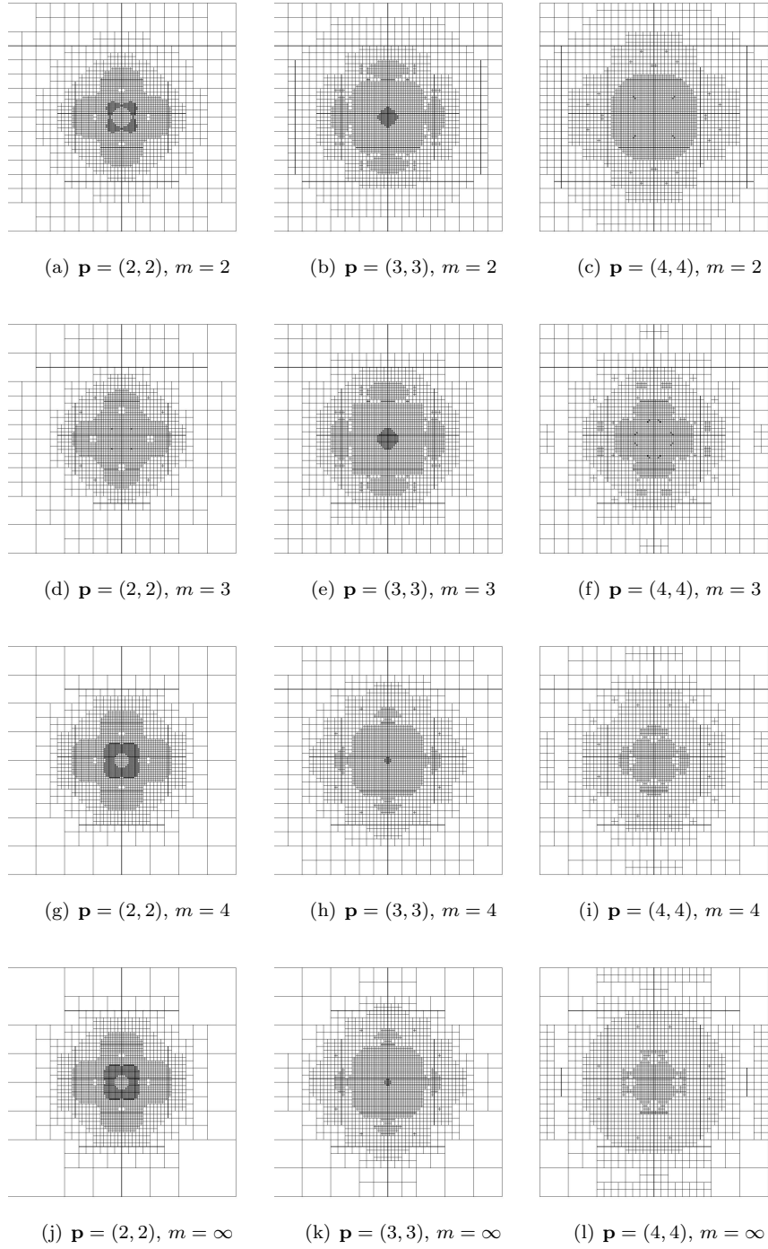
FIGURE 5. Hierarchical meshes obtained for the smooth solution with a peak.
