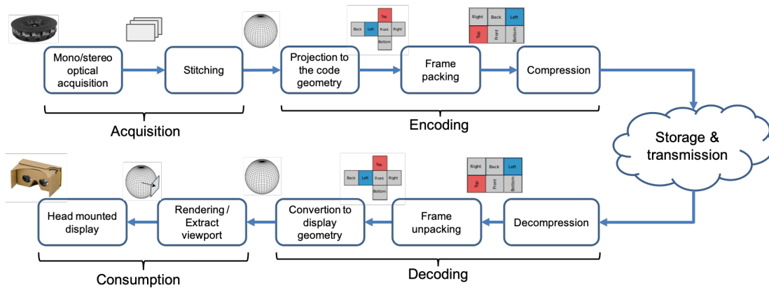
Fig. 1: End-to-end 360-degree video processing pipeline.
