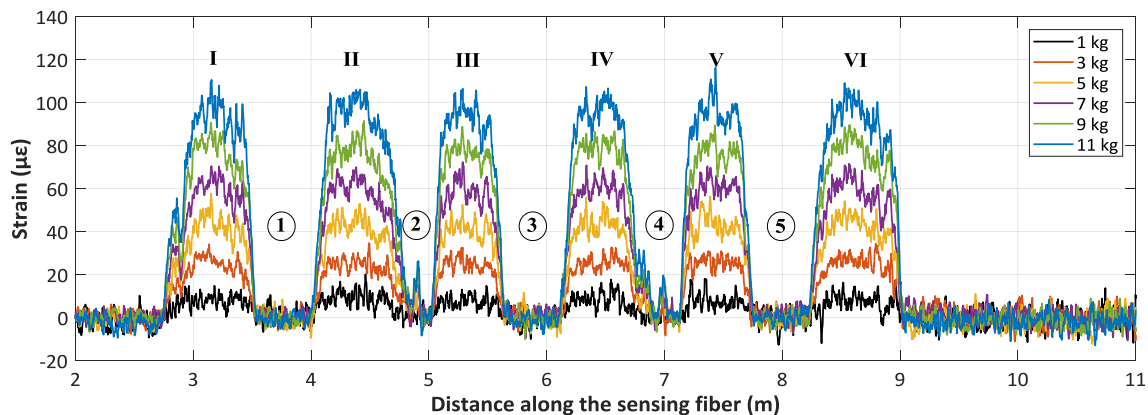
Fig. 5. Experimental distributed OFDR strain response of the CFRP packaging for different loads.
