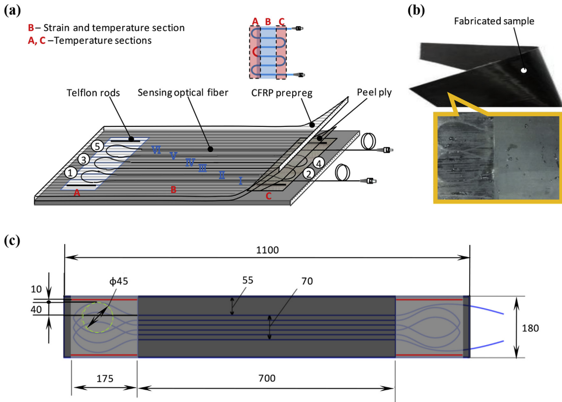
Fig. 2. (a) Schematic of the CFRP packaging with embedded optical fibers for distributed sensing. (b) Fabricated modular CFRP structure. (c) Details of optical fiber layout.
