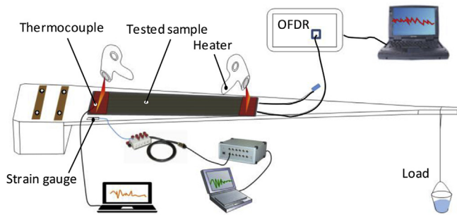
Fig. 3. Schematic diagram of the strain sensing loading test.
