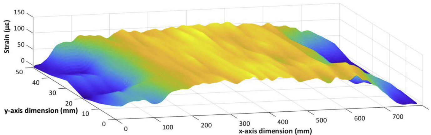
Fig. 7. Retrieved 2D distributed strain profile measured on the CFRP package when the cantilever beam is loaded with 9 kg.
