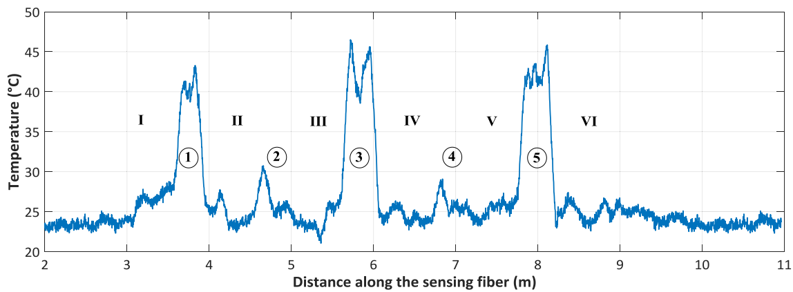
Fig. 4. Experimental distributed OFDR temperature response of the CFRP packaging.
