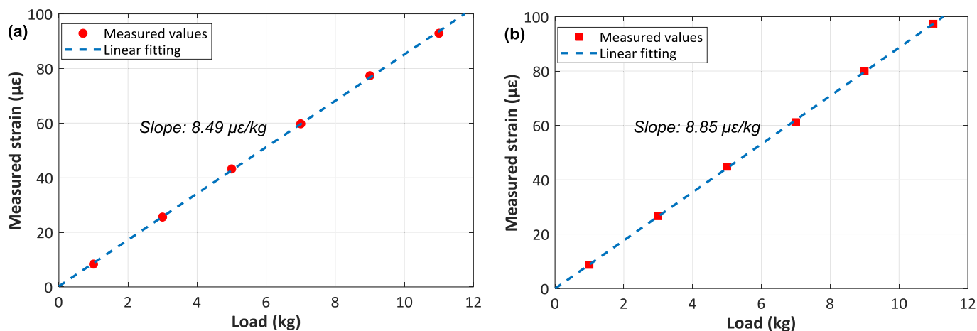
Fig. 6. Measured (average) strain response versus applied load for (a) OFDR sensor with embedded optical fibers in the proposed CFRP packaging, and (b) conventional strain gauges.
