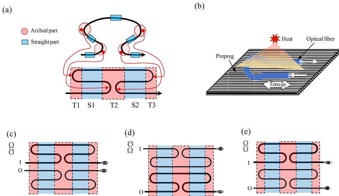
Fig. 1. Schematic of proposed sensing unit. (a) Basic \Omega -shaped fiber to be used to form the sensing structure. (b) Basic sensing cell for both temperature and strain measurements. (c) Back-to-back layout. (d) Face-to-face layout. (e) Sequential stacking layout.
