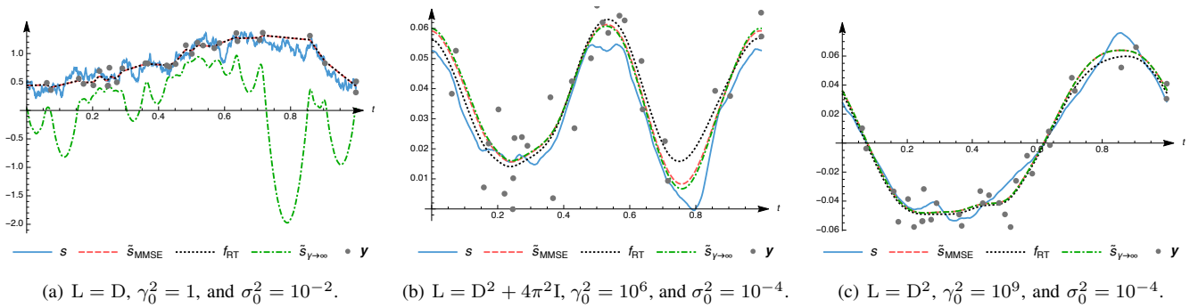
Fig. 4. Illustrations of s \sim \mathcal{GB}(L, \gamma_0^2) , \tilde{s}_{\text{MMSE}} , f_{\text{RT}} , and \tilde{s}_{\gamma \rightarrow \infty} for several operators and values of \gamma_0^2 and \sigma_0^2 . We used M = 30 noisy measurements \mathbf{y} = (y_1, \dots, y_M) .
