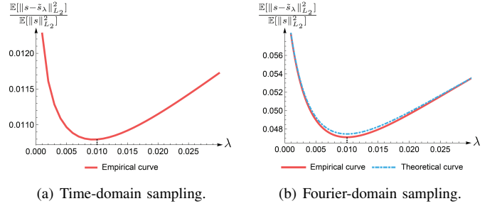
Fig. 3. Evolution of the NMSE in terms of \lambda for s \sim \mathcal{GB}(D+1) for time and Fourier-domain sampling measurements.
