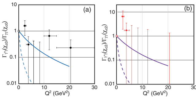
FIG. 13. Q^2 dependence of \Gamma_{\gamma^*\gamma} for the (a) \chi_{c0} and (b) \chi_{c2} mesons normalized to \Gamma_{\gamma\gamma} (at Q^2 = 0 ) [15]. The data point without a dot is based on a zero-event observation, and the upper edge of its error bar corresponds to the value for one event. The overall uncertainties due to the normalization errors of the \Gamma_{\gamma\gamma} \mathcal{B}(K_S^0 K_S^0) are not shown. The solid and dashed curves, respectively, show the SBG [6] prediction and also one motivated by VDM, assuming \rho dominance.
