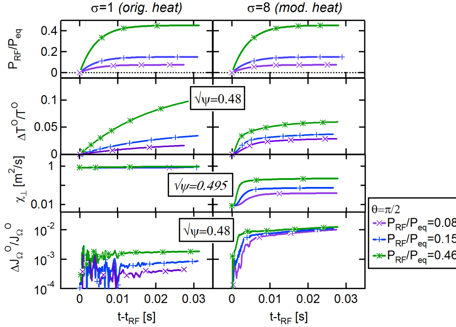
Figure 9. From top to bottom : time evolution of P_{RF}/P_{eq} , \Delta T^O/T^O , perpendicular diffusivity (at \sqrt{\psi} = 0.495 ) and \Delta J_\Omega^O/J_\Omega^O at the island O-point. The stiffness is \sigma = 1 in the left plots (with the original heat source) and \sigma = 8 in the right plots (with the modified one).
