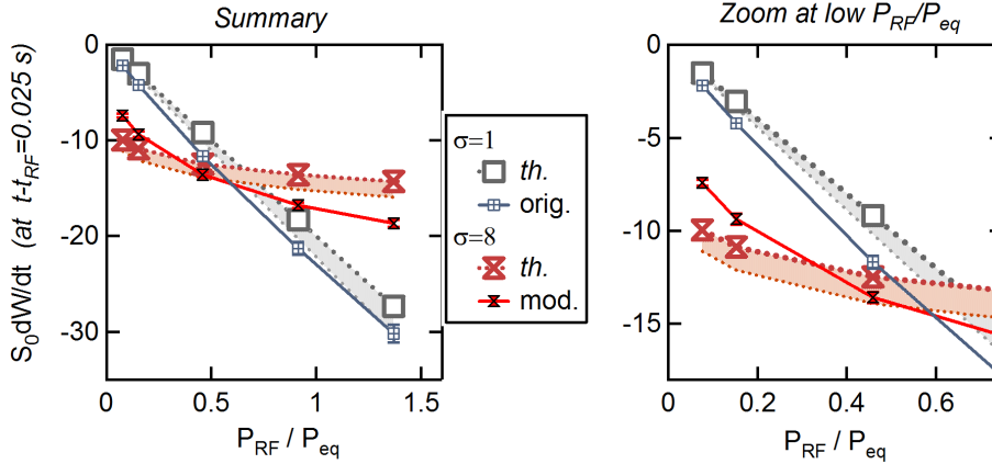
Figure 16. Decay rate of the island at t - t_{RF} = 0.025 s as a function of P_{RF}/P_{eq} for the relevant heat sources (original heat source for \sigma = 1 and modified one for \sigma = 8 ). Right plot: focus on low P_{RF}/P_{eq} values.
