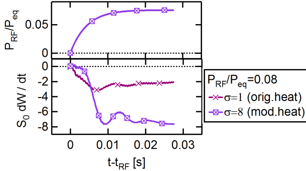
Figure 14. Injected RF power (top) and island decay rate (bottom) for P_{RF}/P_{eq} = 0.08 : comparison between \sigma = 1 and \sigma = 8 .
