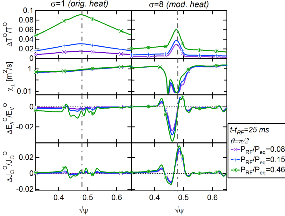
Figure 8. From top to bottom : radial profile (crossing the O-point) of \Delta T^O/T^O , perpendicular diffusivity, \Delta E_{||}^O/E_{||}^O and \Delta J_{\Omega}^O/J_{\Omega}^O . The temperature stiffness is \sigma = 1 in the left plots (with the original heat source) and \sigma = 8 in the right plots (with the modified one). The vertical line is at the radial position of the O-point, \sqrt{\psi} = 0.48 .
