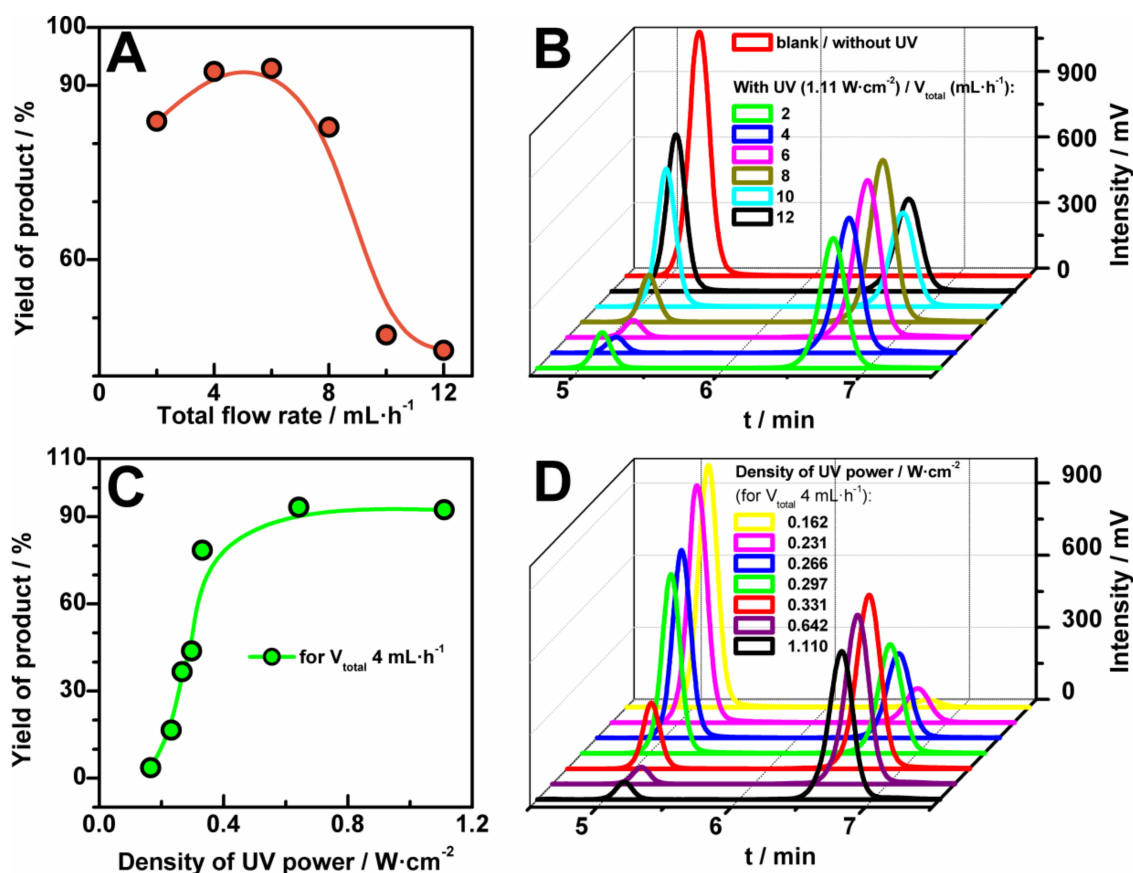
Figure 5. Yield of bromination reaction of 1-indanone ( 1 , 0.25 M) in benzylic position with the use of N-bromosuccinimide ( 2 , 0.26 M) in acetonitrile in the function of flow rate (A) and power of UV lamp (C) and the corresponding High Performance Liquid Chromatography (HPLC) chromatograms (B,D; eluent acetonitrile: water = 60:40). Reaction occurred at room temperature.
