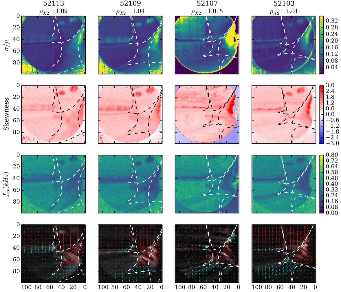
Figure 5. Pixel-wise fluctuation amplitude, skewness, average frequency and apparent flow for each plasma in the \rho_{X2} scan . Separatrices corresponding to the two X-point flux-surfaces are projected onto the image.
