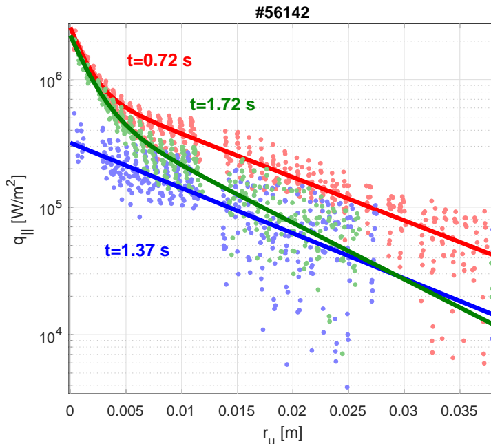
Figure 7: Parallel heat flux radial profiles q_{||}(r_u) before N_2 injection (red dots), for f_{rad} > 70\% (blue dots), and after the gas injection ends (green dots). The fit with Eq. (1) is shown with solid lines.
