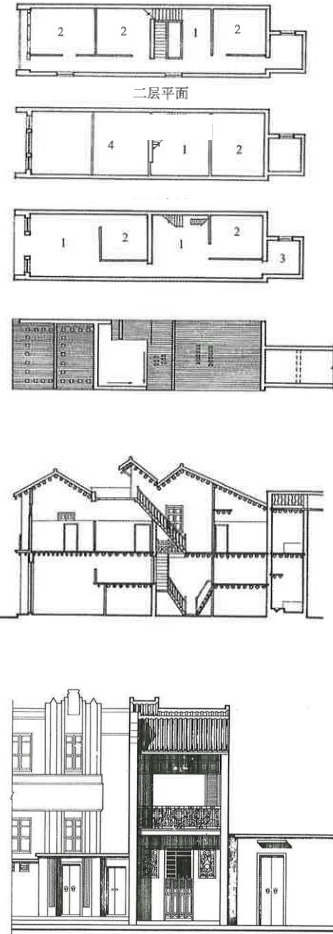
Plan and section of house in Lingnan style, early 20 th century. 2 Lu, Qi
