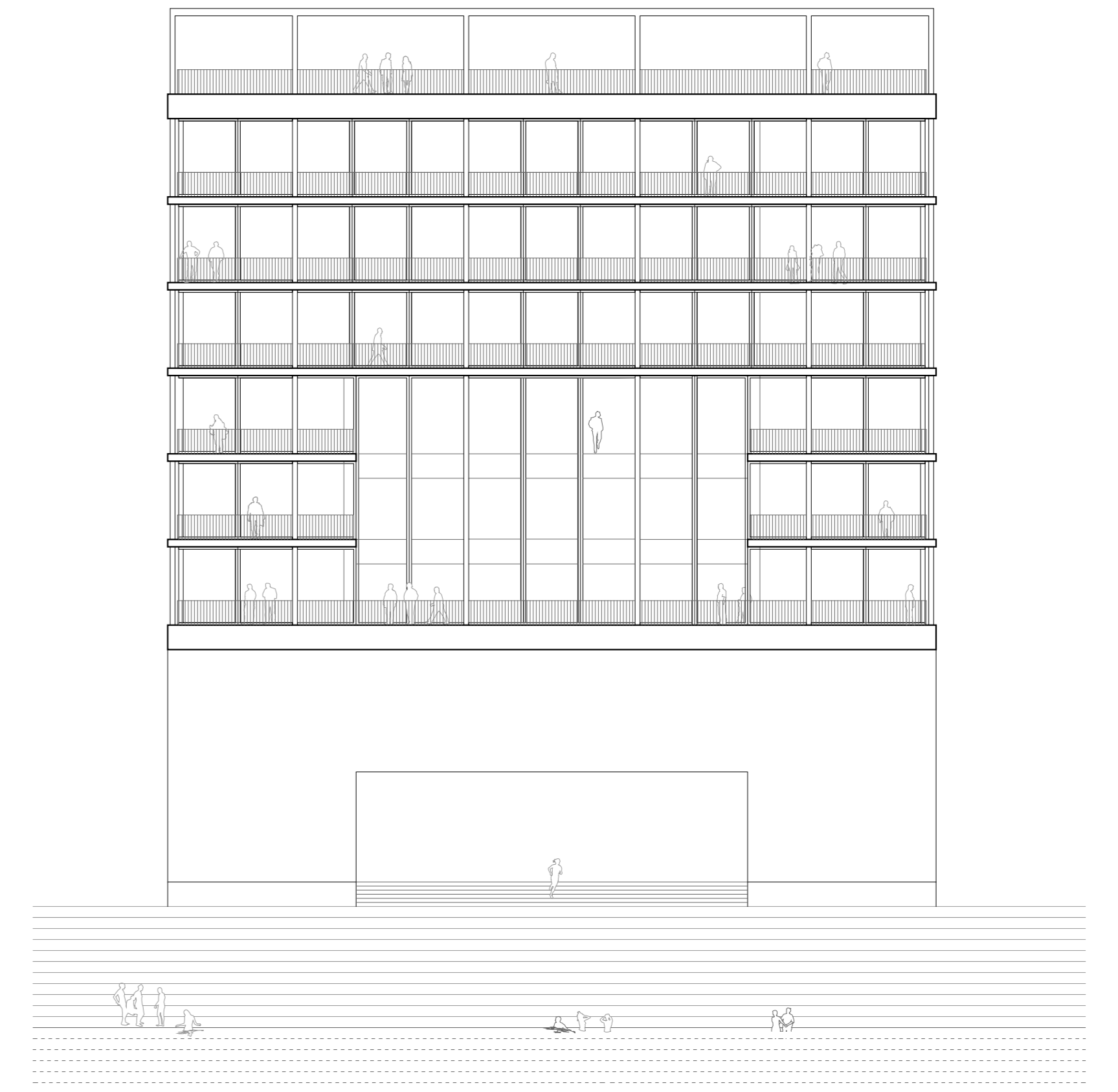
Elevation Coté Mer Echelle 1200
