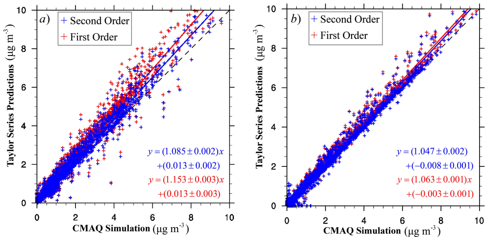
Fig. 8. Comparisons of model simulation and predictions using Taylor series expansions for concentrations of nitrate at 16:00 EDT on 2 January 2004, with (a) a 50 % reduction in \text{NO}_x and (b) a 50 % reduction in \text{SO}_2 . The solid lines reflect the linear regression of the Taylor series predictions against the CMAQ simulation results; the dotted lines represent the area of perfect agreement.
