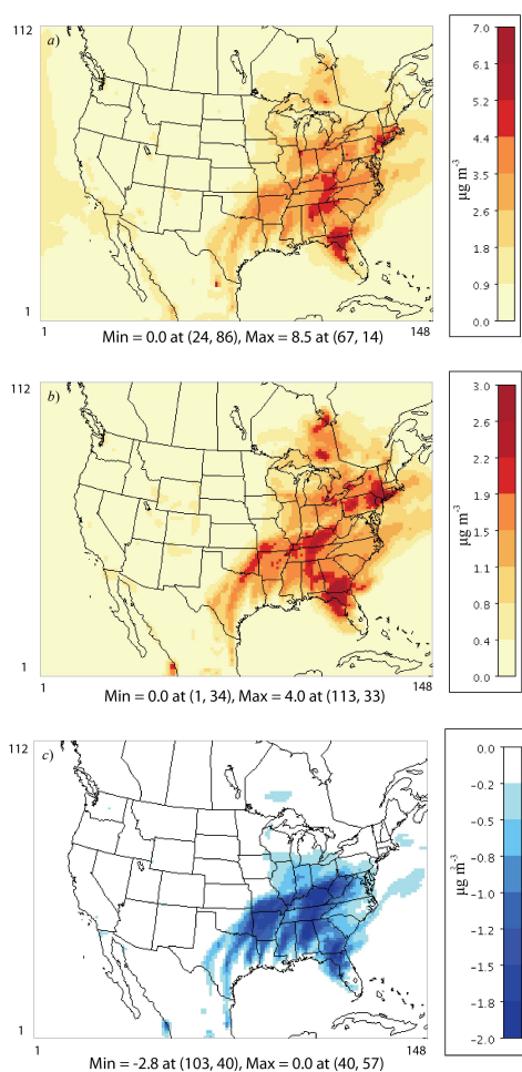
Fig. 4. Spatial distribution of 24-h averages of (a) simulated concentration of sulfate, (b) first- and (c) second-order sensitivities of sulfate to \text{SO}_2 at surface layer on 3 January 2004.
