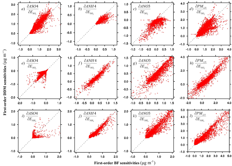
Fig. 5. Comparison of first-order sensitivities of sulfate, ammonium, nitrate, and PM_{2.5} to SO_2 , NO_x , and NH_3 calculated by HDDM-3D/PM and BF at surface layer on 2 January 2004. ASO_4 , ANH_4 , and ANO_3 denote aerosol sulfate, aerosol ammonium, and aerosol nitrate, respectively. Each plot represents one sensitivity coefficient that is labeled on the upper left of the plot. The dashed line is the one-to-one line indicating perfect agreement.
