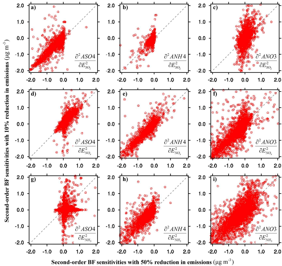
Fig. 7. Comparison of second-order BF sensitivities calculated with 10 % and 50 % perturbation in emissions using CMAQ simulation on 2 January 2004 at surface layer. ASO4, ANH4, and ANO3 denote aerosol sulfate, aerosol ammonium, and aerosol nitrate, respectively.
