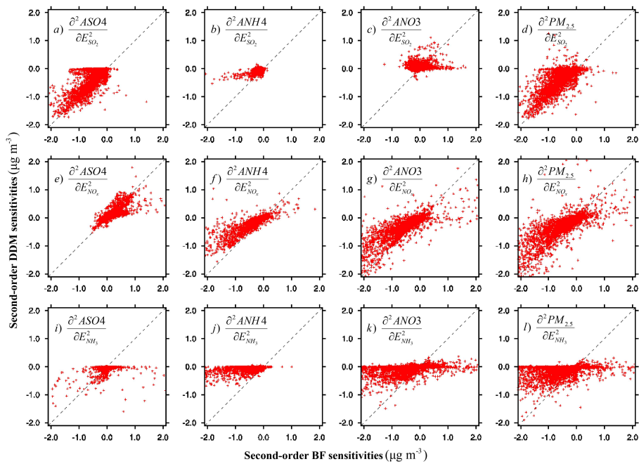
Fig. 6. Comparison of second-order sensitivities of sulfate, ammonium, nitrate, and PM_{2.5} to SO_2 , NO_x , and NH_3 calculated by HDDM-3D/PM and BF at surface layer on 2 January 2004. ASO_4 , ANH_4 , and ANO_3 denote aerosol sulfate, aerosol ammonium, and aerosol nitrate, respectively. Each plot represents one sensitivity coefficient that is labeled on the upper left of the plot. The dashed line is the one-to-one line indicating perfect agreement.
