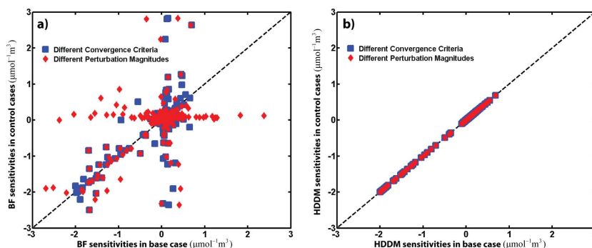
Fig. 3. Second-order sensitivity coefficients of aerosol nitrate to total sulfate in stand-alone ISORROPIA calculated by (a) BF and (b) HDDM under three conditions: (1) base case, where the perturbation used by BF ( \Delta p ) = 1% and the convergence criteria of ISORROPIA ( \Delta\eta ) = 1 \times 10^{-10} ; 2) control case 1 (blue squares) with \Delta p = 1% and \Delta\eta = 1 \times 10^{-3} ; and 3) control case 2 (red diamonds) with \Delta p = 0.1% and \Delta\eta = 1 \times 10^{-10} . The default value of the convergence criteria for ISORROPIA is 1 \times 10^{-6} . Results from the two control cases are compared to those from the base case. The dashed line is the one-to-one line.
