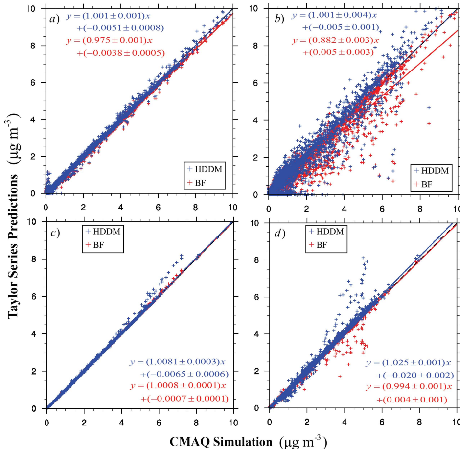
Fig. 9. Comparisons of model simulation and predictions using Taylor series expansions with HDDM and BF sensitivities for concentrations of nitrate with (a) 20 % and (b) 100 % reductions in domain-wide SO 2 emissions rates and concentrations of sulfate with (c) 20 % and (d) 100 % reductions in domain-wide NH 3 emissions rates at 16:00 EDT on 2 January 2004. BF sensitivities are from a 50 % perturbation. The solid lines reflect the linear regression of the Taylor series predictions against the CMAQ simulation results; the dotted lines represent the area of perfect agreement.
