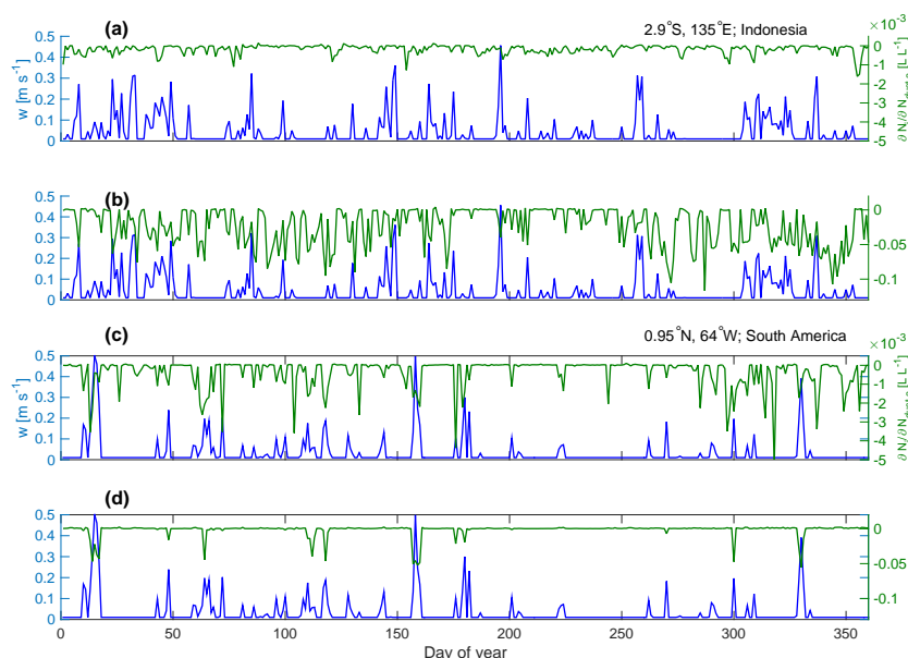
Figure 6. Time series of accumulation-mode dust number sensitivities (green, in \text{LL}^{-1} ) and input updraft velocities (blue, in \text{m s}^{-1} ) over Indonesia at 2.9^\circ \text{ S} , 135^\circ \text{ E} for (a) PDA08 and (b) PDA13; and over South America at 0.95^\circ \text{ N} , 64^\circ \text{ W} for (c) PDA08 and (d) PDA13.
