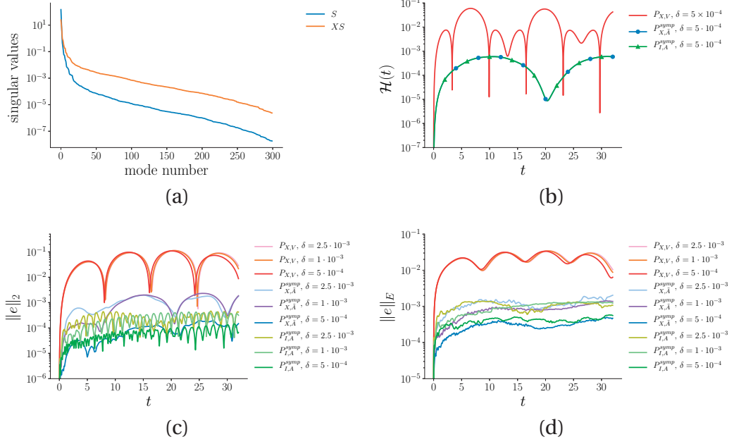
Figure 5.3 – Numerical results related to the beam with cavity. (a) the decay of the singular values, (b) conservation of the Hamiltonian, (c) error with respect to the 2-norm, (d) error with respect to the energy norm.
