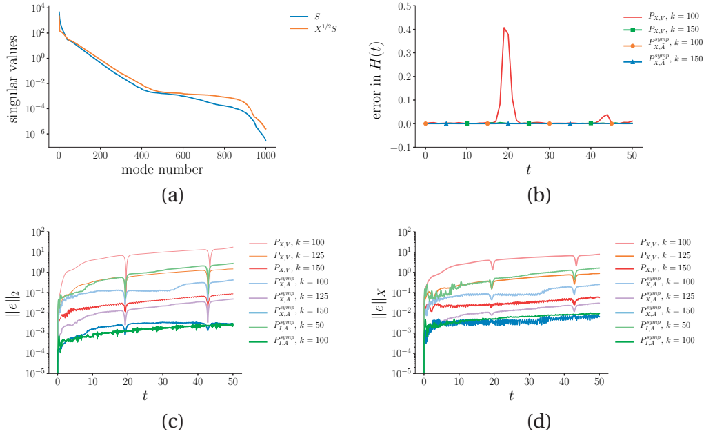
Figure 5.4 – Numerical results related to the sine-Gordon equation. (a) the decay of the singular values, (b) the error in the Hamiltonian, (c) the error with respect to the 2-norm, (d) the error with respect to the energy norm.
