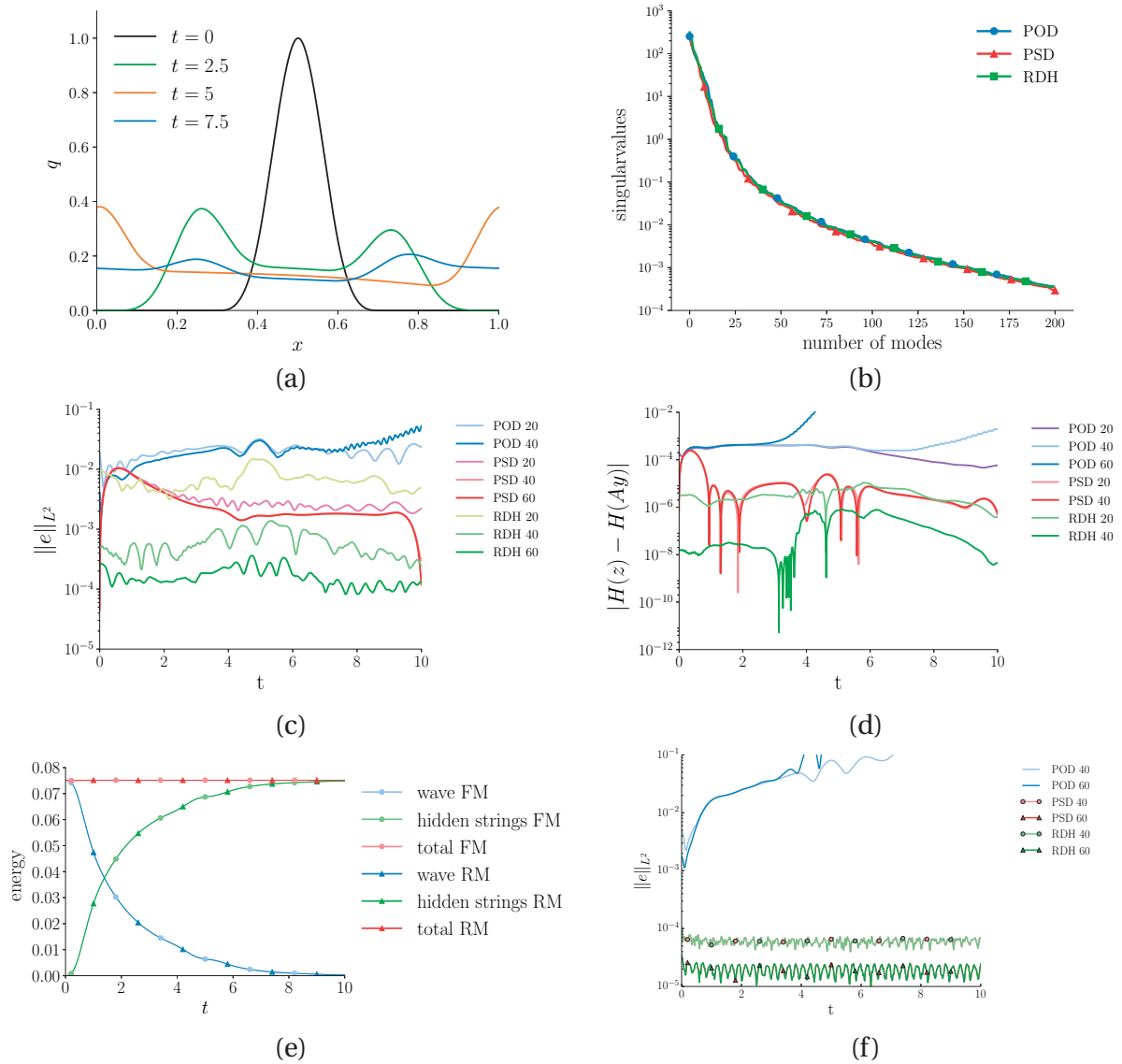
Figure 6.1 – (a) The solution to the original dissipative wave equation (6.25), (b) The decay of the singular values for the POD, the PSD, and the RDH methods, (c) The L^2 -error for the different methods, (d) Evolution of error in the Hamiltonian for different methods, (e) Energy preservation of the Hamiltonian extension for the original and the reduced system. “FM” and “RM” refer to the full model and the reduced model, respectively. (f) The L^2 -error between the solution to the reduced system and the full system in a near-zero dissipation regime.
