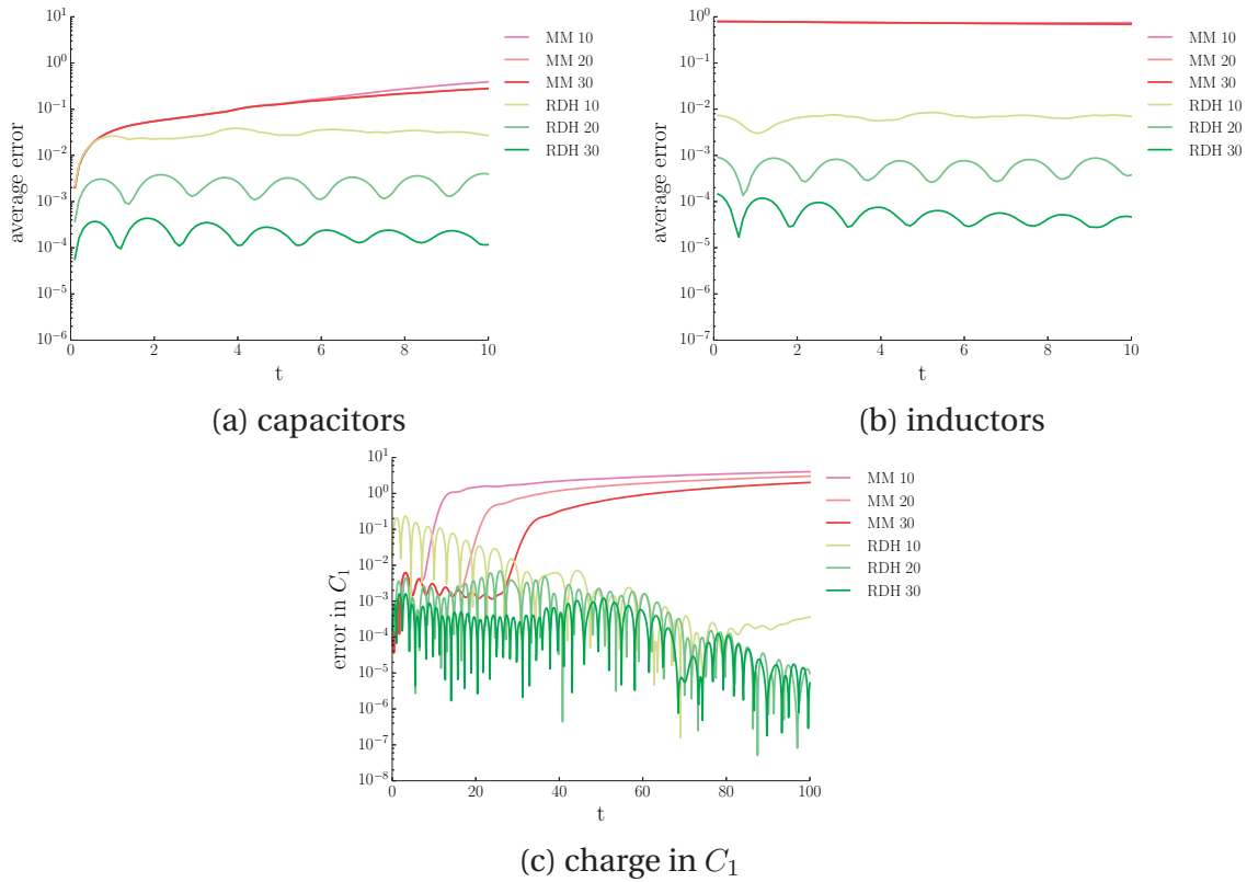
Figure 6.4 – Error between the full model and the reduced model obtained by the reduced dissipative Hamiltonian method “RDH” and the moment matching method “MM”. (a) The average temporal error of charge in capacitors. (b) the average temporal error of the flux in inductors. (c) The error in C_1 .
