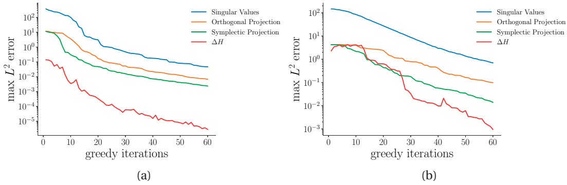
Figure 4.5 – (a) Convergence of the greedy method for the wave equation. (b) Convergence of the greedy method for the nonlinear Schrödinger equation equation.
