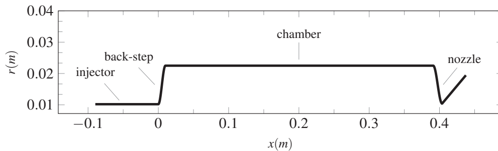
Figure 7.12 – Geometry of quasi-1D CVRC model.
