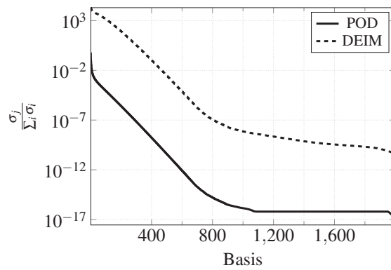
Figure 7.10 – Decay of the singular values of the snapshot matrix related to POD and DEIM algorithms for the 1D compressible Euler problem.
