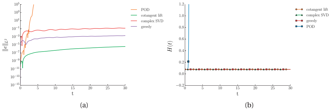
Figure 4.2 – (a) The L^2 -error between the solution of the full system and the reduced system for different model reduction methods for t \in [0, 30] . (b) Plot of the Hamiltonian function for t \in [0, 30] .
