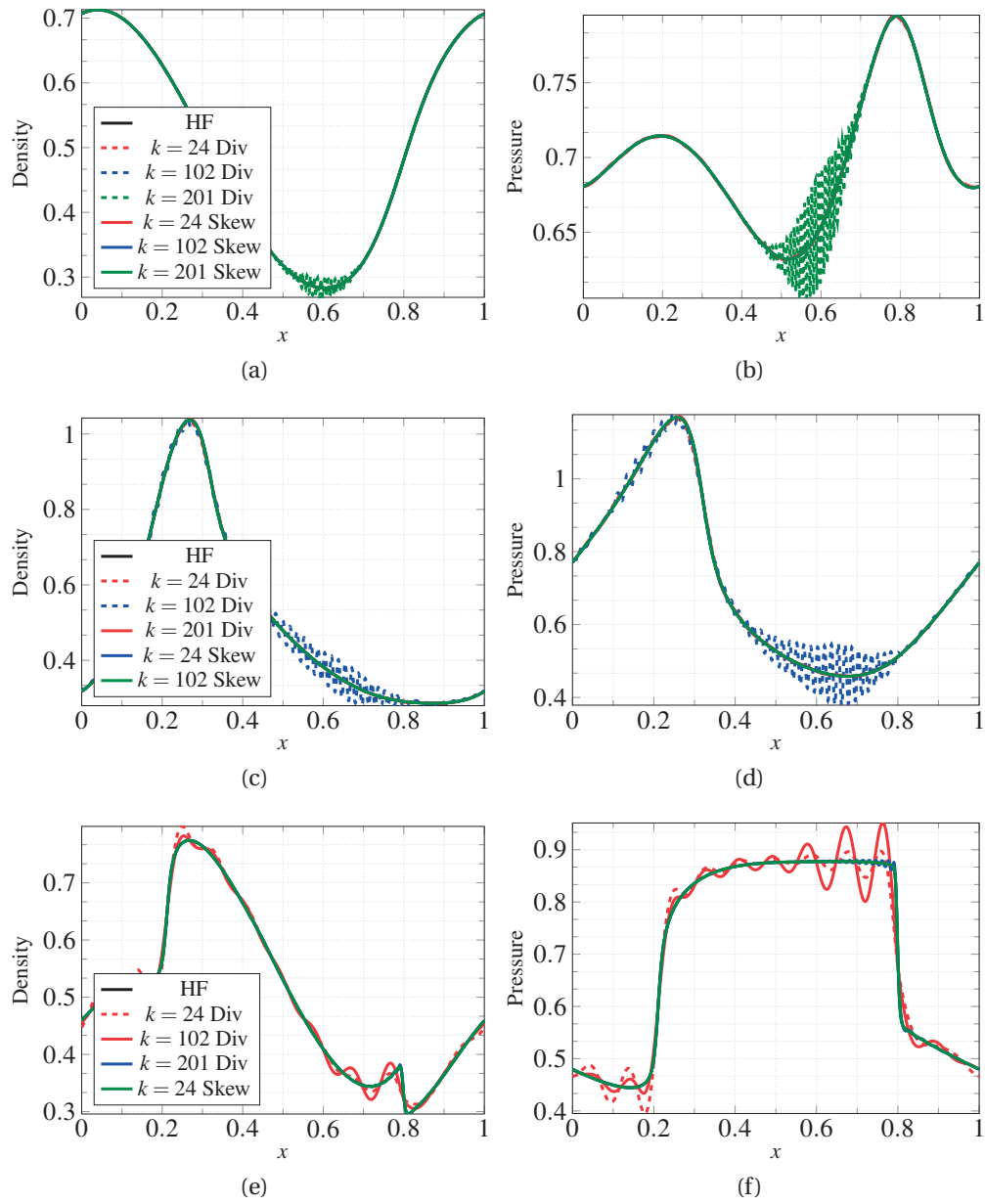
Figure 7.9 – Qualitative comparison between different formulations for the reduced model in terms of density (left) and pressure (right) at t = 0.1, 0.3 and 1s . Results for the advective formulation are not showed here because the related reduced solutions are unstable after a few time steps.
