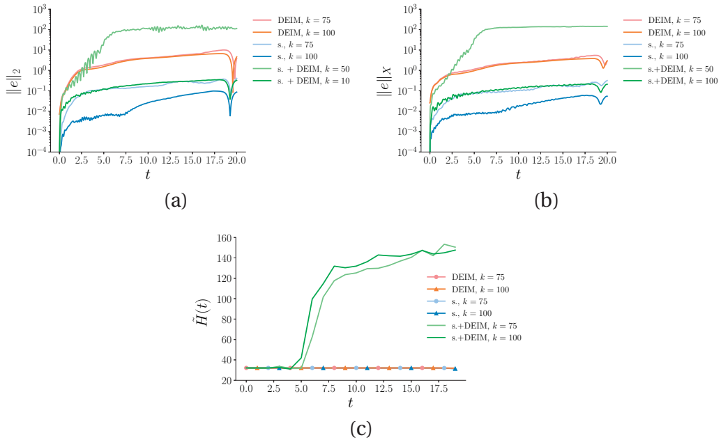
Figure 5.5 – Numerical results related to the sine-Gordon equation with efficient evaluation of the nonlinear terms. Here, “DEIM” indicates classical model reduction with the DEIM, “s.+DEIM” indicates symplectic model reduction with the DEIM and “s.” indicates symplectic model reduction with symplectic treatment of the nonlinear term. (a) error with respect to the Euclidean norm, (b) error with respect to the X -norm, (c) error in the Hamiltonian.
