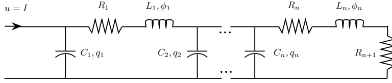
Figure 6.3 – n -dimensional ladder network
