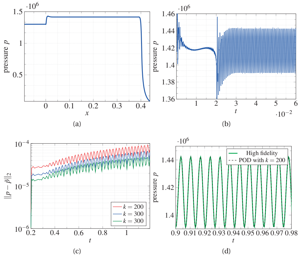
Figure 7.13 – (a) Pressure profile of the steady state. (b) Oscillatory mode of pressure located at x = 0.36 for the unsteady flow. (c) Relative error between the high-fidelity and approximated pressure. (d) Approximation of the oscillations.
