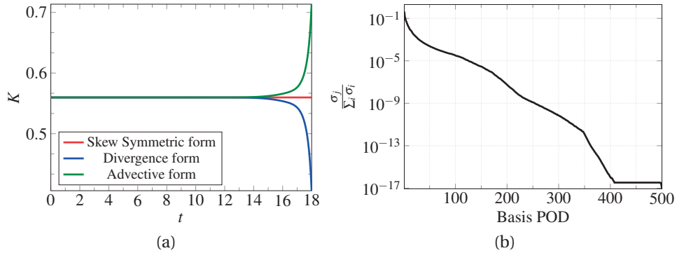
Figure 7.1 – (a) The kinetic energy K for the advective, divergence and the skew-symmetric formulations. (b) The decay of the singular values for the vortex merging.
