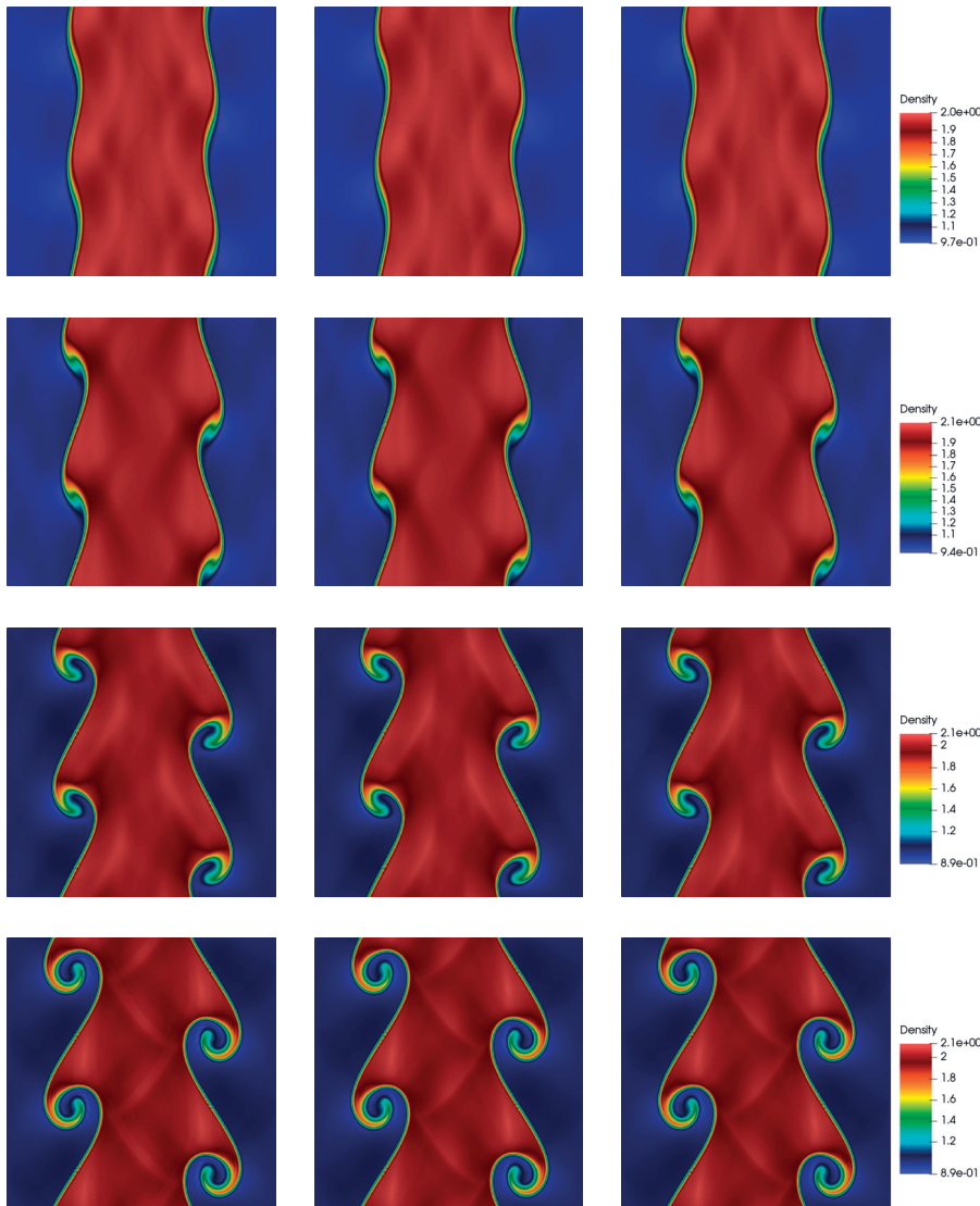
Figure 7.6 – Solutions of the Kelvin-Helmholtz problem at t = \{0.4, 0.6, 0.8, 1\} . From left to right we show the solution of the reduced model with k = 200 , k = 500 and the high fidelity solution.
