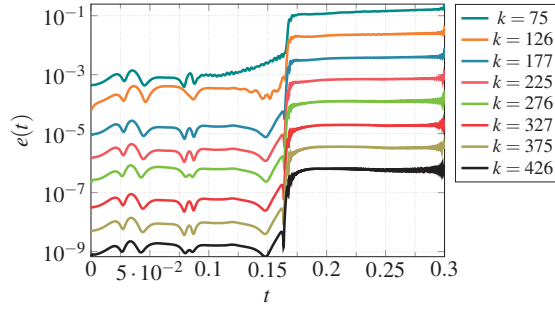
Figure 7.8 – Evolution in time of the error between the high fidelity solution of the 1D compressible Euler and the reduced solution for different number of basis k . As error measure we consider e(t) = \sqrt{\|\mathbf{r} - \mathbf{r}^r\|^2 + \|\mathbf{ur} - \mathbf{ur}^r\|^2 + \|\mathbf{p} - \mathbf{p}^r\|^2} .
