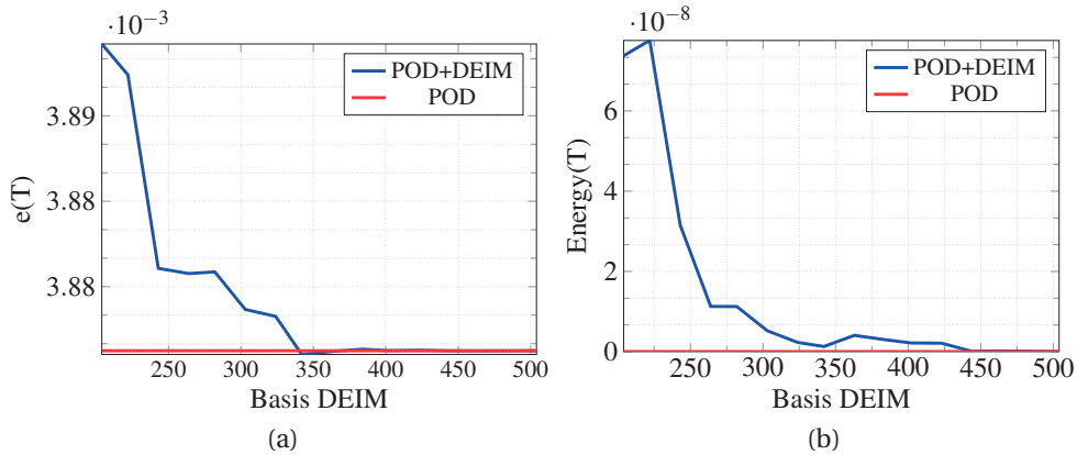
Figure 7.11 – Comparison between standard POD and POD with DEIM treatment of the nonlinear term in terms of the error (a) and the total energy (b).
