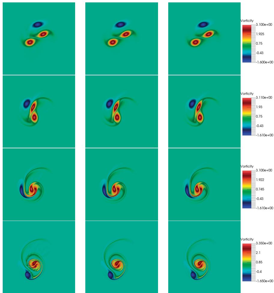
Figure 7.2 – Snapshots of the high-fidelity system and the reduced system at t = \{4, 8, 12, 18\} . From left to right: the solution of the reduced model with k = 17 , k = 35 and the high fidelity solution.
