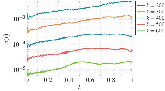
Figure 7.4 – Evolution in time of the error between the high fidelity solution of the Kelvin-Helmoltz and the reduced solution for different number of basis k . As error measure we use e(t) = \sqrt{\|\mathbf{r} - \mathbf{r}^r\|^2 + \|\mathbf{u}_x \mathbf{r} - \mathbf{u}_x \mathbf{r}^r\|^2 + \|\mathbf{u}_y \mathbf{r} - \mathbf{u}_y \mathbf{r}^r\|^2 + \|\mathbf{p} - \mathbf{p}^r\|^2} .
