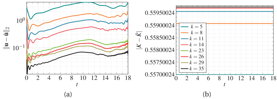
Figure 7.3 – (a) Evolution of L_2 error in velocity, between the high-fidelity system and the reduced system. (b) Conservation of the kinetic energy.
