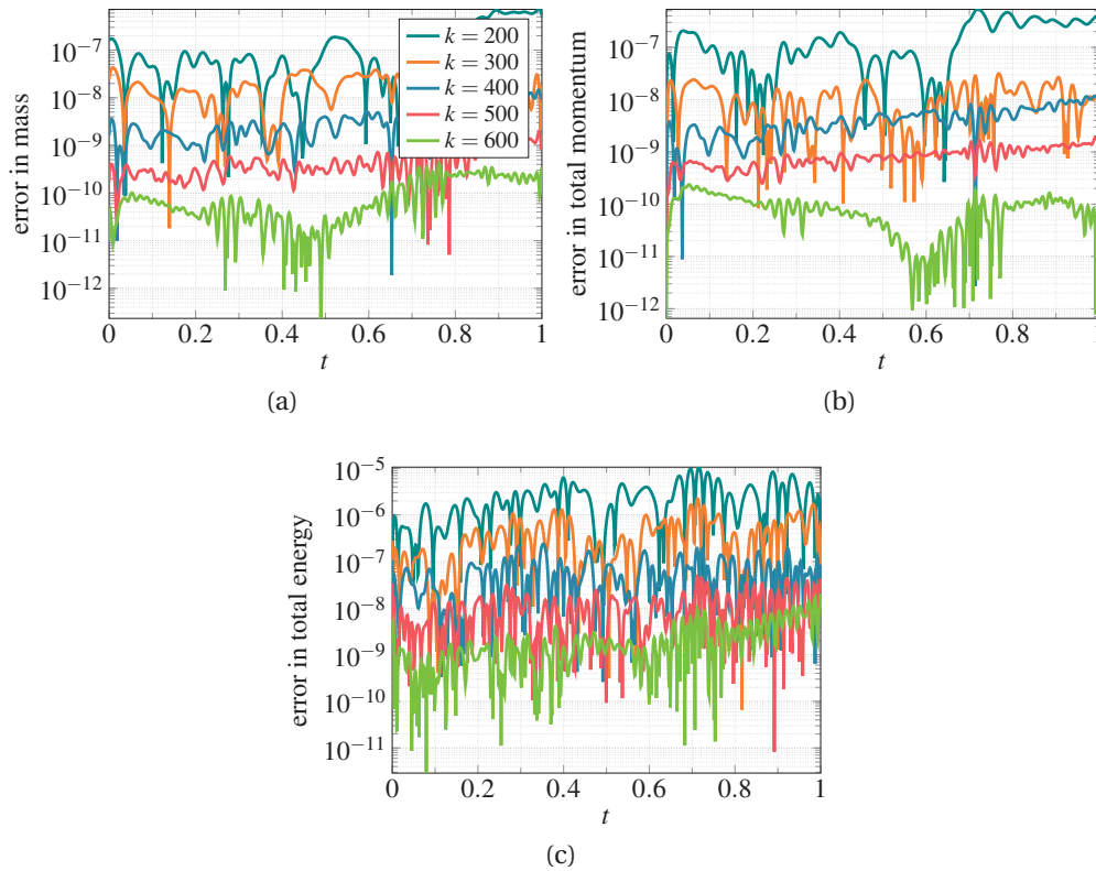
Figure 7.5 – Difference between the high fidelity solution of the Kelvin-Helmholtz problem and the reduced solution of the mass (a), the momentum (b), and the total energy (c).
