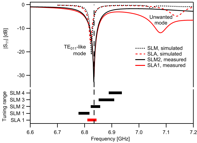
FIG. 3. Top: Measured (solid lines) and simulated (dashed lines) S_{11} curves for the SLM (black) and SLA (red) cavities. Due to calibration differences in the AM processes, the nominal gap sizes of prototypes SLA1 and SLM2 differ by 50\ \mu\text{m} . Bottom: Measured frequency tuning ranges. Frequency tuning between the four SLM cavities (black bars) is achieved by gap sizes differing by 50\ \mu\text{m} each. Frequency fine tuning of each single cavity, over the frequency range indicated by the widths of the horizontal bars, is achieved by varying the dielectric loading of the cavity via adjusting the cell position.
