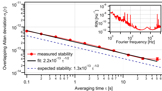
FIG. 7. Measured clock stability in the Ramsey mode. Inset: signal noise for the detection phase.
