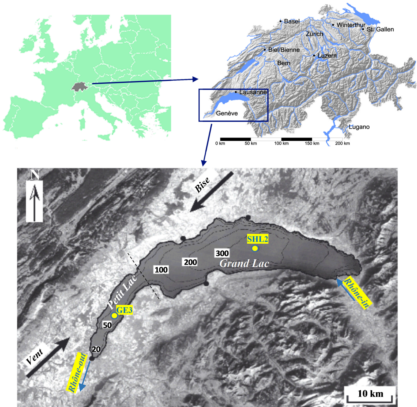
Fig. 1. Location and bathymetry of Lake Geneva, adapted from a public domain satellite image (NASA World Wind, last accessed 5 July 2018) and bathymetry data (SwissTopo, last accessed 5 July 2018). SHL2 (46.45°N, 6.59°E) and GE3 (46.3°N, 6.22°E) are two monitoring locations in the lake used for model calibration and validation. The thick black arrows indicate the direction of the two dominant strong winds over lake called Bise and Vent . Rhône-in and Rhône-out show the lake's main river inflow and outflow locations, respectively.
