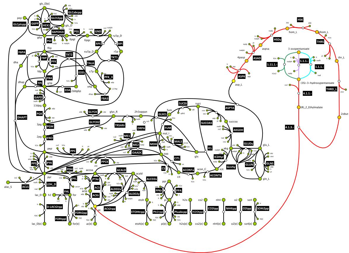
F1: Three alternative ways to produce 3OXPNT from acetate through 2 intermediate metabolites: 2-ethylmalate and 3-hydroxypentanoate.
