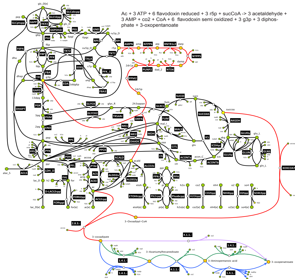
F2: Three different pathways from acetate to 3OXPNNT sharing the same lumped reaction.
