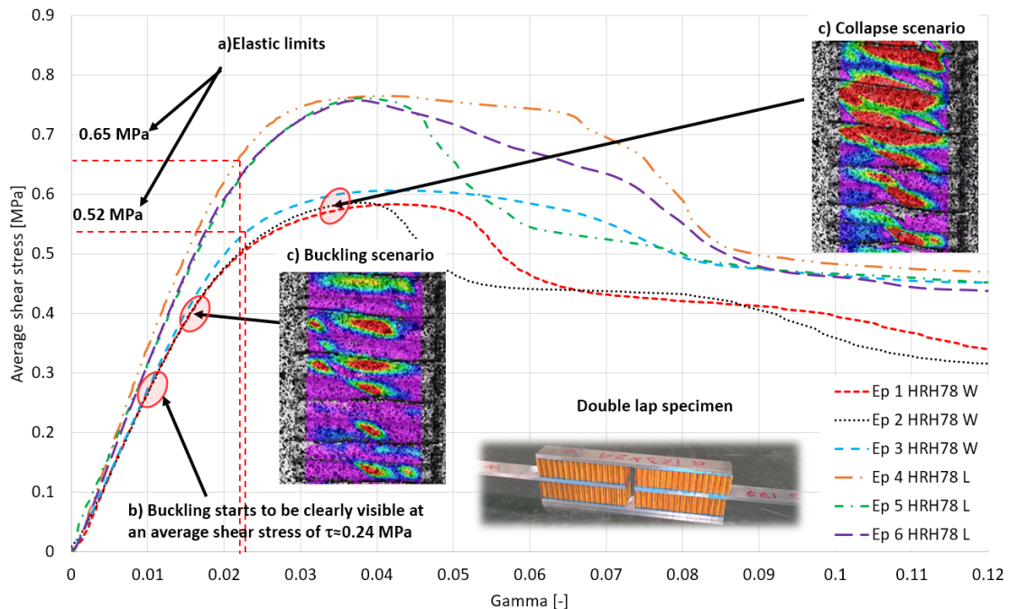
Fig. 1: Description of the shear behavior of the HRH-78 Nomex Honeycomb core (a) The elastic limits were detected trough an incremental cyclic testing, (b) The buckling of the cells is detected at a relatively low shear stress, (c) Buckling scenario of collapsing and non-collapsing cells.
