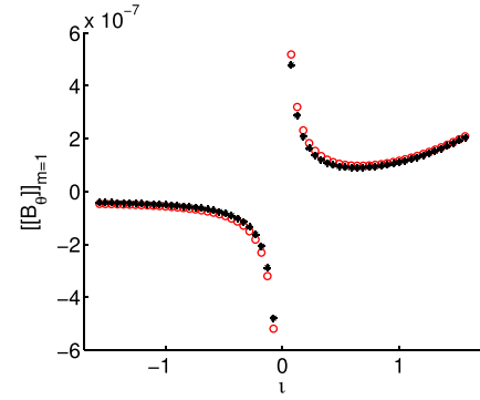
FIG. 12. Discontinuity in the m=1 component of the poloidal field at each interface as a function of the corresponding rotational transform \iota for a MRxMHD equilibrium with N_V = 63 , R_{3,1} = 10^{-2} , p_0 = 10^{-3} , and X = 0.04 . A divergent current is established around \iota_{res} = 0 . Red circles are from SPEC and black stars are from the linearized model.
