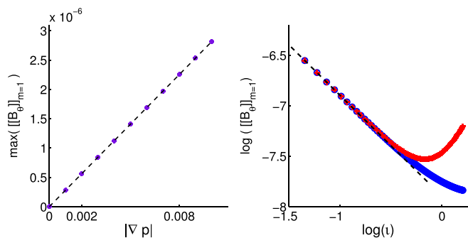
FIG. 8. Left: magnitude of [B_\theta]_{m=1} across a fixed interface, as a function of the pressure gradient |\nabla p| \equiv p_0 , showing a linear relation (black dashed line has slope 1). Right: log-scale plot of the negative (blue circles) and positive (red crosses) sides of the curve in Fig. 7, showing a 1/t divergence (black dashed line has slope -1 ) near the resonant rational surface.
