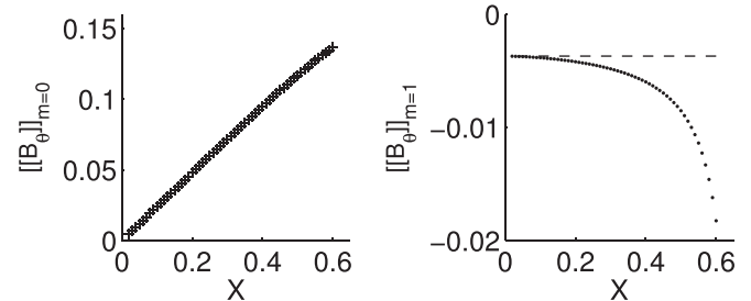
FIG. 5. Discontinuity in the poloidal field as a function of the sequence parameter X . Left: m = 0 component, which is expected to be zero in the limit X \rightarrow 0 , see Eq. (20). Right: m = 1 component, expected to be finite in the limit X \rightarrow 0 , with a theoretical value given by Eq. (21) (dashed line).
