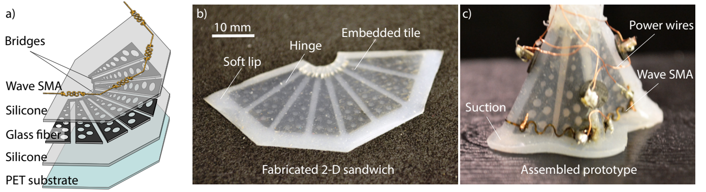
Fig. 5. The rapid 2-D layer-by-layer fabrication process of the suction gripper and the fabricated prototypes in 2-D and 3-D. a) The rigid fiberglass tiles are embedded between two silicone rubber layers to enable flexure hinges, conformity and sealing at the gripper opening. The wave SMA actuators are mounted lastly onto the sandwich. b) The fabricated 2-D prototype without wave SMA actuator layer, which was folded and assembled to 3-D c).
