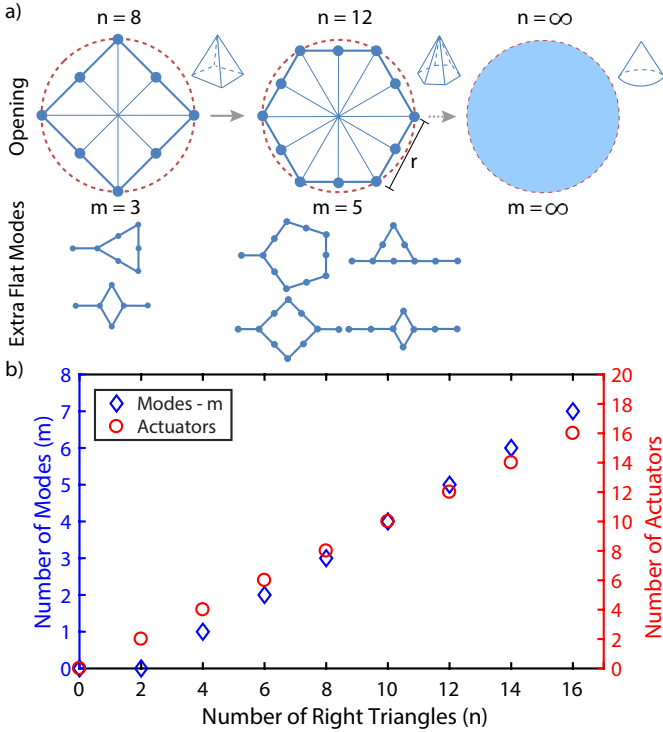
Fig. 2. The geometric approximation of a conic shape suction cup by rigid triangles connected with compliant hinges and producing number of cross-sectional opening modes by folding. a) Connecting eight or higher number of right triangles in chain approximates the conic shape of the cup. Multiple modes of flat opening can be produced if some tiles are folded in valley or mountain fashion. Increasing the number of triangles n produces more flat opening modes m , hence more accurate representation of the conic suction cup. b) The number of tiles versus the number of actuators and achievable number of modes plot. The number of tiles requires equal number of actuators, whereas the number of flat opening modes is proportional to the tile number.
