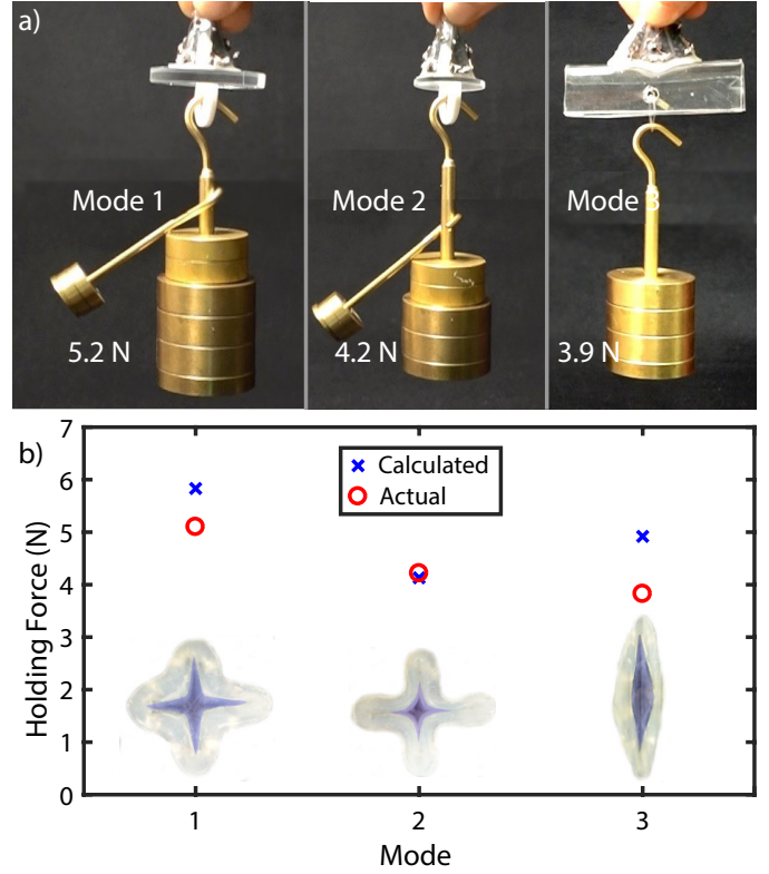
Fig. 9. The origami suction gripper holding force measurement test and plots. a) For Mode 1, the gripper is attached to a flat round plate ( d = 43 mm) with a hole to hook weights. The gripper can lift up to 5.2 N weight. Similarly, a smaller plate ( d = 29 mm) is used for lifting weights up to 4.2 N with Mode 2. Finally, a bent acrylic plate with 9.5 mm curvature is employed for hooking weights up to 3.9 N in Mode 3. b) The comparison between the actual and calculated holding forces in each mode. The expected forces are calculated by measuring the actual gripper opening area, shaded with blue, on a transparent surface at -80 kPa vacuum pressure. The actual value is slightly lower than the analytic one for Mode 1 and comparably lower for Mode 3 due to imperfect sealing.
