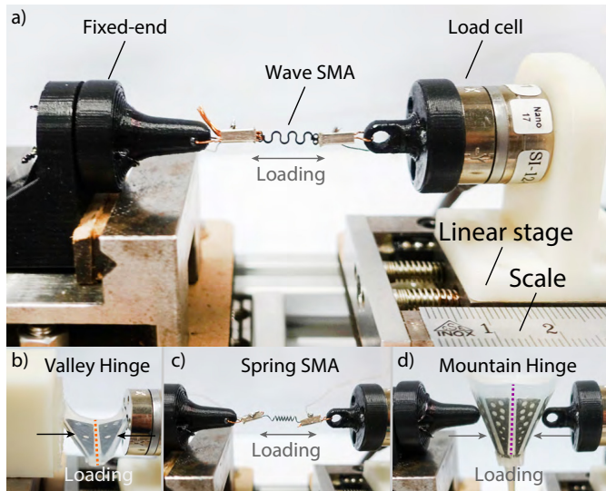
Fig. 6. The blocked force measurement setup for SMA actuators and rubber hinges. a) The wave SMA actuator is clamped to the fixed part at one end and to the moving part with a load cell at the other end. The linear stage is moved to multiple positions and the actuator forces are measured for both austenite and martensite phases. b) The valley hinge force characterization by bending. c) The spring SMA mounted to the setup is tested similarly as the wave SMA. d) The mountain hinge force measurement by compressing with two point tips from both sides.
