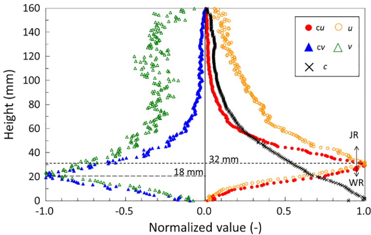
Fig. 9. Normalized sediment mass flux, velocity and concentration distribution at t = 0-10 and 10-20 s at x = 5.22 m.
