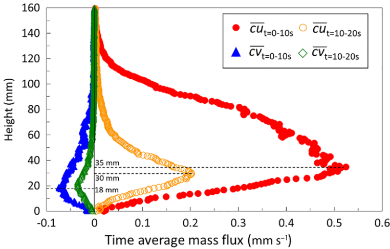
Fig. 8. Time-averaged sediment mass flux distribution at t = 0-10 and 10-20 s at x = 5.22 m.
