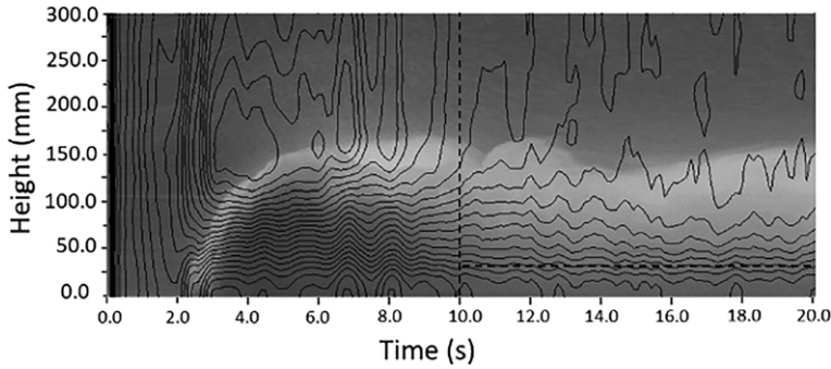
Fig. 5. Timeline image and equipotential lines at x = 5.22 m. One pixel corresponds to 0.04 s \times 0.31 mm. Vertical and horizontal dashed lines represent the boundary of the head and body, and the horizontal velocity maximum.
