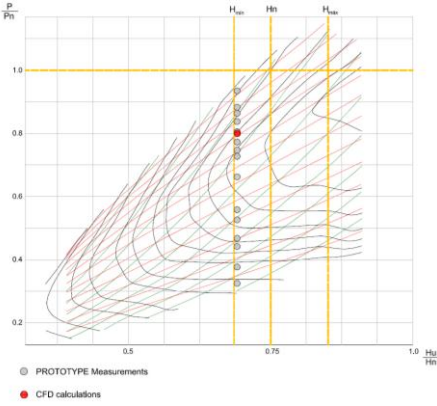
Fig. 2 Point measured and simulated over the discharge hill.
