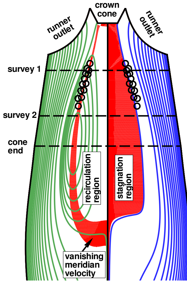
Figure 5. Streamline pattern and the location of the vortex rope. Numerical results for axisymmetric turbulent flow model without SRM (left half-plane) and with SRM (right half-plane).
