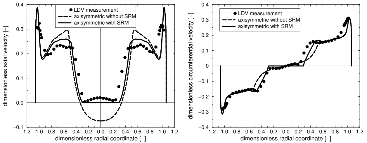
Figure 3. Axial and circumferential velocity profiles on the upstream survey section S1.
