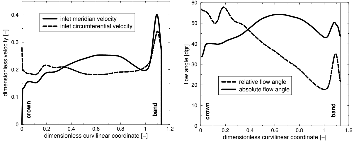
Figure 2. Velocity profile and flow angle on the inlet section of the computational domain from Figure 1, with curvilinear coordinate running from crown to band.
