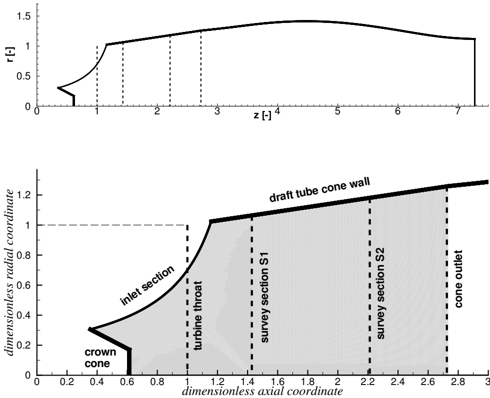
Figure 1. Computational domain in a meridian half plane.
