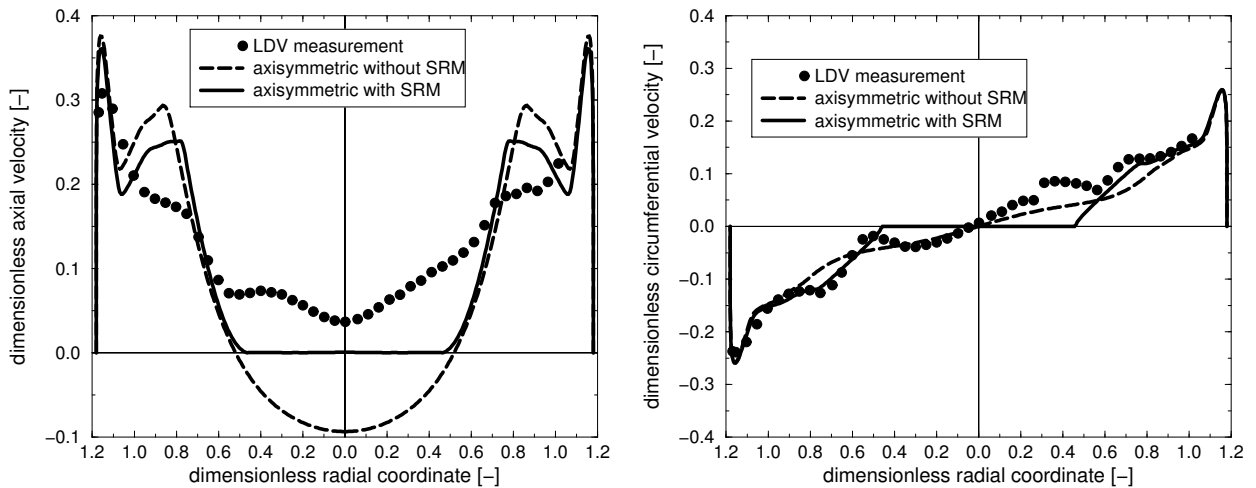
Figure 4. Axial and circumferential velocity profiles on the downstream survey section S2.
