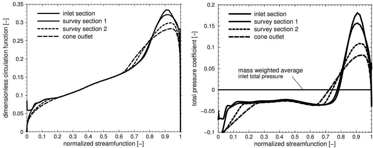
Figure 6. Dimensionless circulation function C(\psi) (left) and total pressure \rho E(\psi) , respectively, versus the normalized streamfunction.
