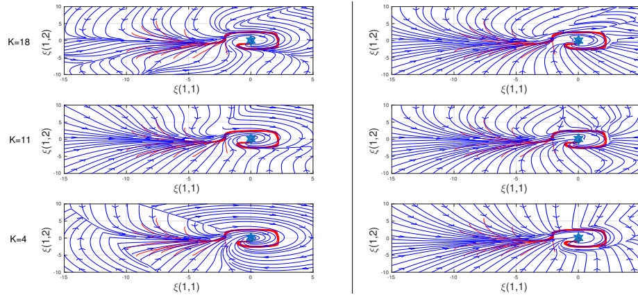
(c) The third set of motions. For K = 4 and K = 11 , SEDS fails to encode the straight line motions near the target as the cyclic motions are dominating.
