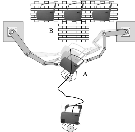
(b) Synchronous Multi-Arm Task-Space Behavior.
