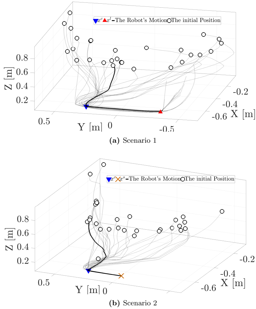
Figure 5.8: Spatial variational of the initial, contact and leaving/stopping points. Experimental results verify that the contact is stable and the robot touches the surface at the desired points.
