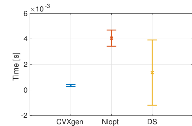
(a) Computation time comparison
