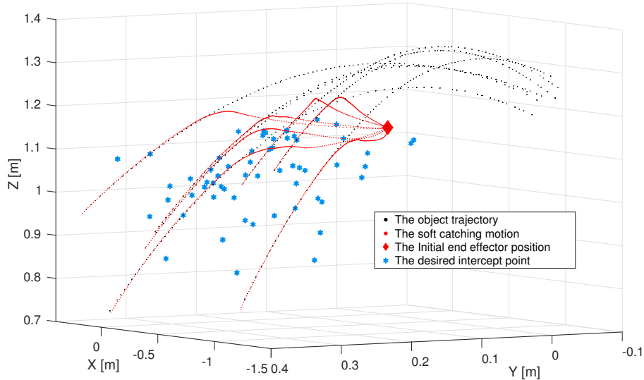
Figure 3.10: The final intercept points in the soft catching experiments. The initial position of the palm is [-0.05 \ 0.00 \ 1.134] m. For clarity of the illustration, only seven examples of the soft catching motions and the object trajectories are shown. The object trajectories are plotted from the first points till the stop points. The first point is the first object position which is used for predicting the feasible intercept position. The experimental results verifies that the catching motion intercepts the object at the desired point with the desired velocity.
