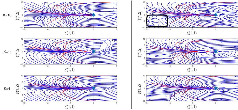
(a) The first set of motions. For K = 4 and K = 18 , SEDS fails to encode the non-linear motions near the target and approximate them with a straight line. As it is highlighted by a box, Algorithm 3.2a results in a jerky motions for K = 18 .
