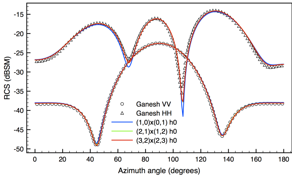
Figure 18: Radar cross section profile for NASA almond geometry: 1.19GHz, horizontal and vertical polarization. Reference data obtained from [19].
