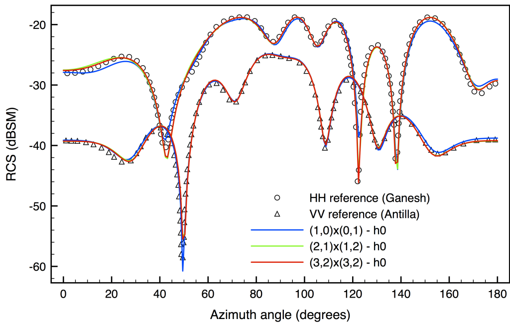
Figure 20: Radar cross section profile for NASA almond geometry: 3GHz, horizontal and vertical polarization. Reference data obtained from [19, 4].
