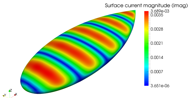
Figure 21: Magnitude of imaginary component of surface current over the NASA almond geometry: vertically polarised planewave of 3GHz travelling in the positive x -direction, mesh h_0 .
