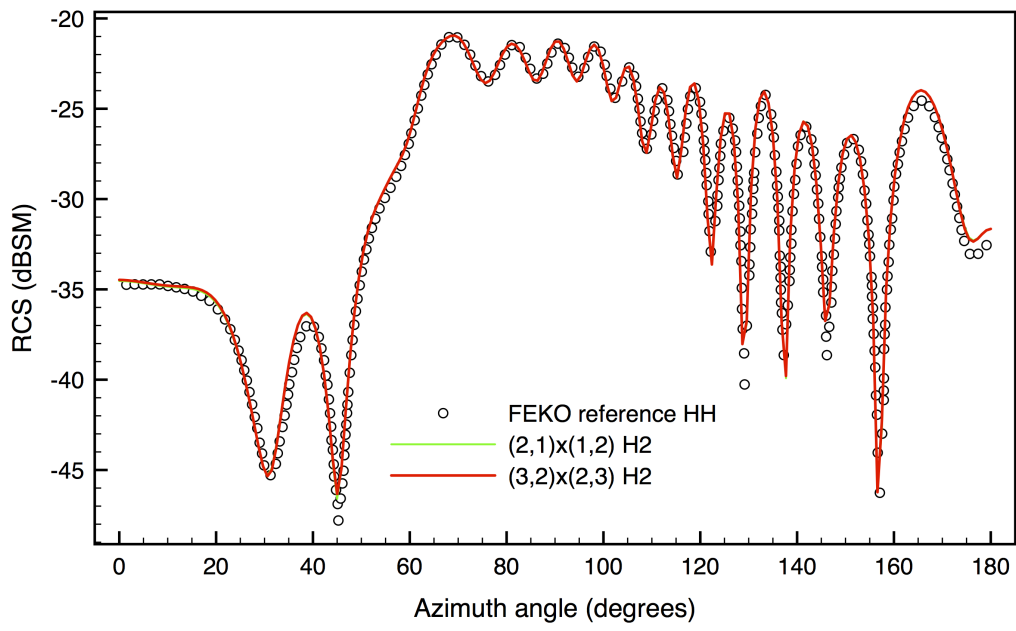
Figure 22: Radar cross section profile for NASA almond geometry: 7GHz, horizontal polarization. Reference data obtained from [2].
