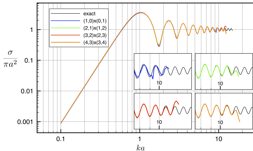
Figure 11: Normalised RCS values for a PEC sphere computed for increasing wavenumber with div-conforming B-splines of varying degree, mesh h_3
