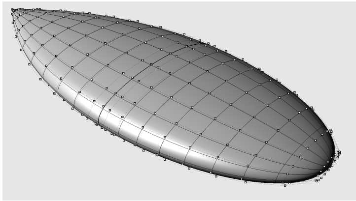
Figure 17: The NASA almond geometry represented by four bicubic NURBS patches with two degenerate points.
