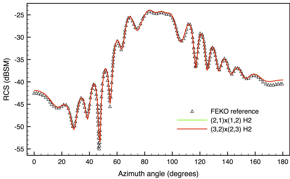
Figure 23: Radar cross section profile for NASA almond geometry: 7GHz, vertical polarization. Reference data obtained from [2].
