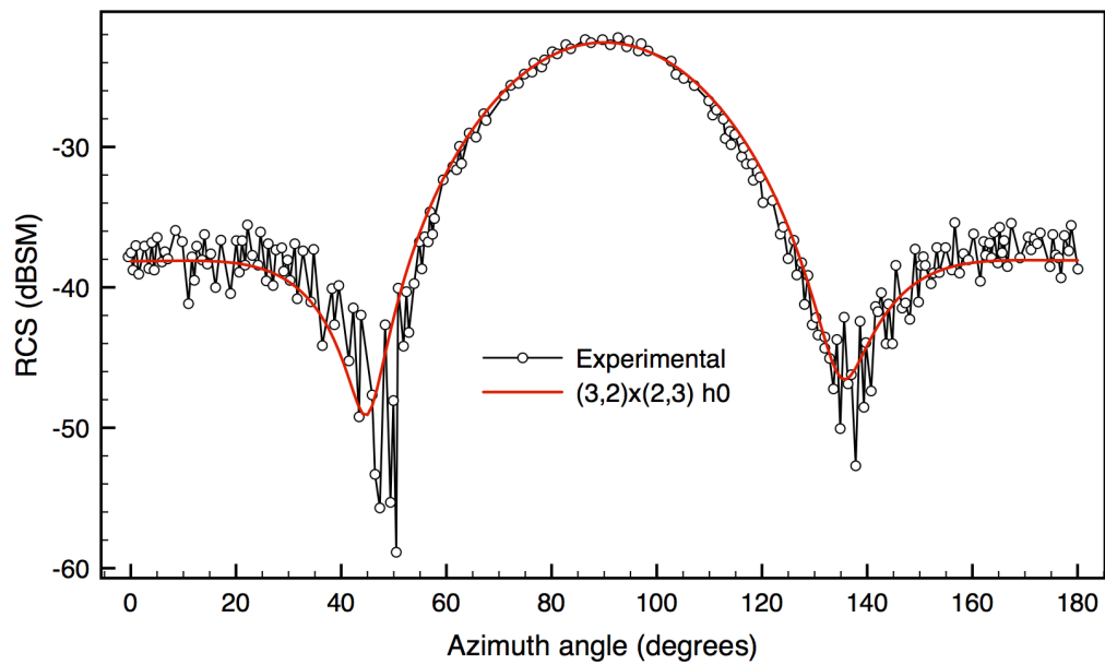
Figure 19: Comparison of experimental and numerical radar cross section profile for NASA almond geometry: 1.19GHz vertical polarization. Experimental reference data obtained from [41].
