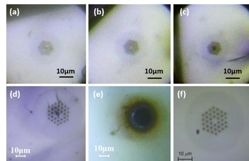
Fig. 3. (a)–(c) Optical image of waist facets after fiber fuse on various locations. (d) Core void due to fiber fuse. (e) Purely thermal induced damage on input facet. (f) Intact facet.
