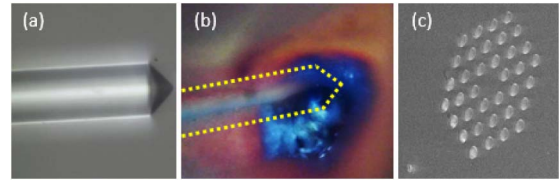
Fig. 6. (a) Input lens fiber before fuse happened. (b) Input lensed fiber coated by ChG after fiber fuse; lensed fiber is out of focus to better image the deposited ChG. (c) SEM image of the input facet of T-PCF2, showing no trace of damage on this facet.
