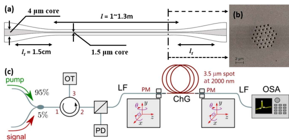
Fig. 1. (a) Geometry of the GeAsSe PCF (not to scale), (b) SEM image of a facet in taper waist, (c) laser setup for parametric conversion test. OT, optical terminator; PD, photodetector; LF, lensed fiber; OSA, optical spectrum analyzer; PM, polarization maintaining (fiber).
