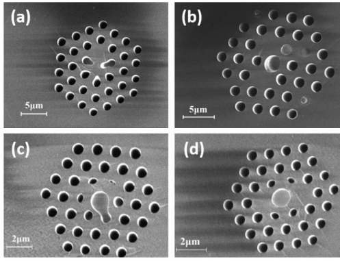
Fig. 4. (a) SEM image of a facet on output transition region of taper 1, close to the start point of fiber fuse; (b) SEM image of the facet from Fig. 3(d); (c) and (d) SEM image of two facets inside the taper waist; shallow bottoms can be seen by using the in-lens detector.
