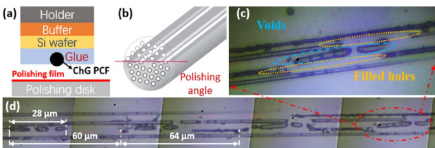
Fig. 5. (a) Sketch of the polishing assembly. (b) Polishing angle of the segment. (c) Composed image of the “opened” fiber. Note the clear periodicity of voids. (d) Enlarged image of voids' top-view.
