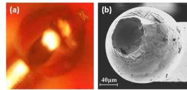
Fig. 2. (a) ChG sphere on the PCF input facet. Note the high reflection from the sphere surface. (b) SEM image of (a); the “crater” came from collision with the lensed fiber.
