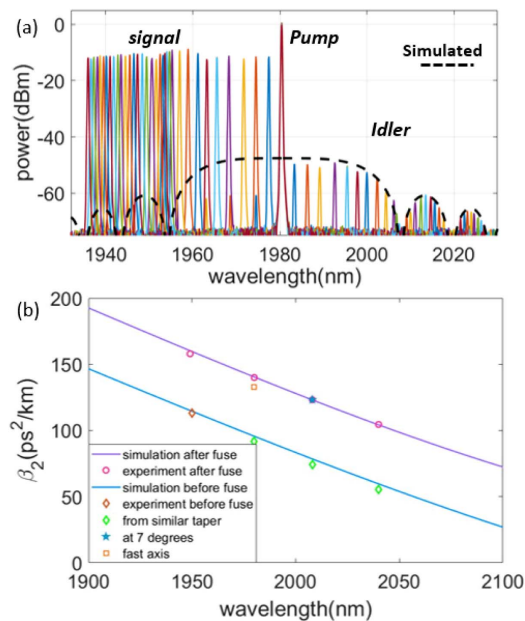
Fig. 7. (a) Superimposed spectrum of signal sweep with theoretical fitting from Eq. (2), about 5-mW pump and 0.3-mW signal power coupled into fiber. (b) Comparison of dispersion before and after fuse.
