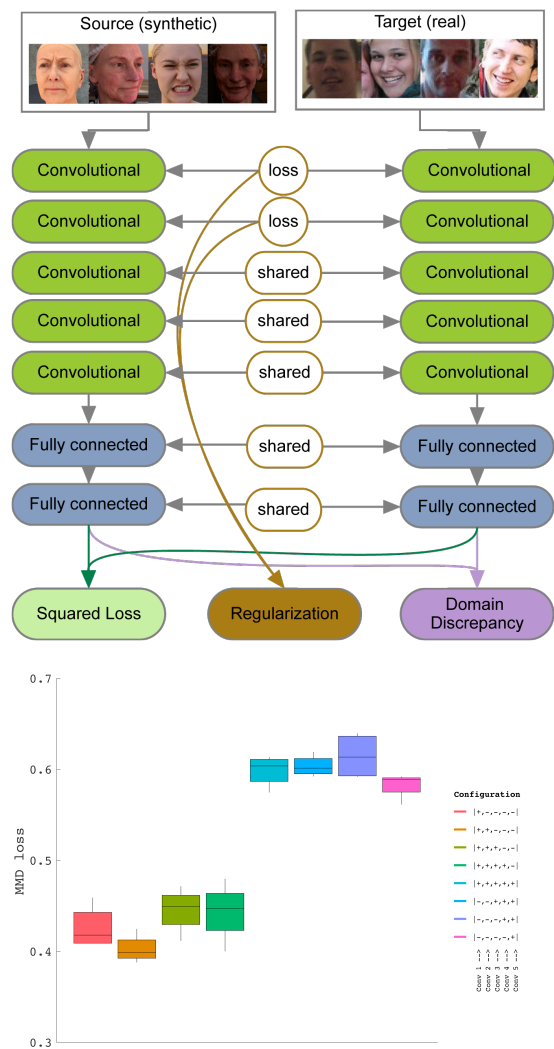
Fig. 11. [TOP] Network architecture for facial pose estimation. [BOTTOM] Network architecture selection. '-' and '+' denote that the weights of the corresponding layers are shared and stream-specific, respectively.
