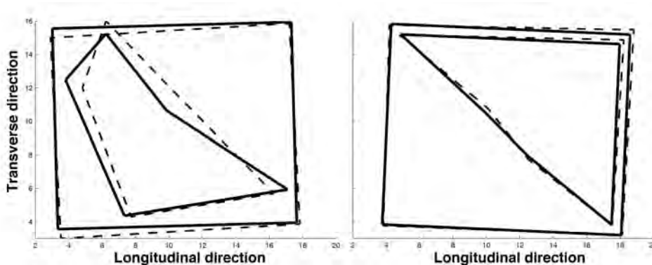
Figure 7. Second mode shape of the 5th story of the structure in test 1 (left) and 3 (right): the inner lines are arbitrarily connecting the recording points, whereas the outer rectangle represents the outer walls of the building. Dashed lines connect the points of the observed modal shape and solid lines correspond to an average rigid body motion of the slab assumed non-deformed
