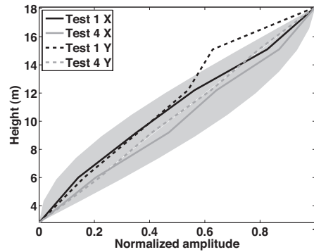
Figure 6. Comparison of the modal shapes in elevation between the first and the fourth test. The grey-shaded area represents the area between the Euler-Bernoulli (pure bending, upper limit) and the pure shear (lower limit) beams (see also [26])
