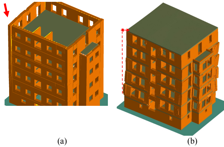
Figure 12. Typical damage mechanisms associated to DG5 in the numerical model of the URM building (a) before and (b) after retrofitting
