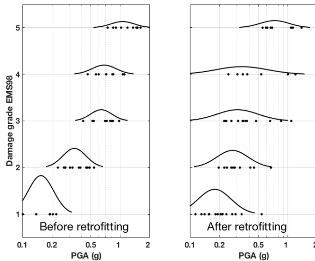
Figure 13. Lognormal distribution of the peak ground acceleration values for each damage grade
