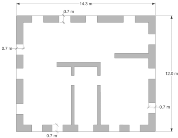
Figure 2. Plan view of the tested building with main dimensions.
