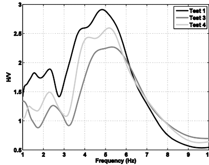
Figure 8. Horizontal to Vertical Spectral Ratios of the soil recordings of the first, third and fourth tests
