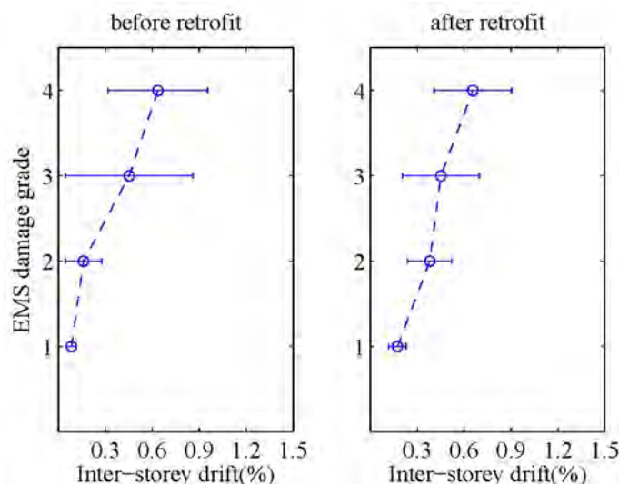
Figure 15. Mean plus/minus one standard deviation for the inter-storey drift at each DG
