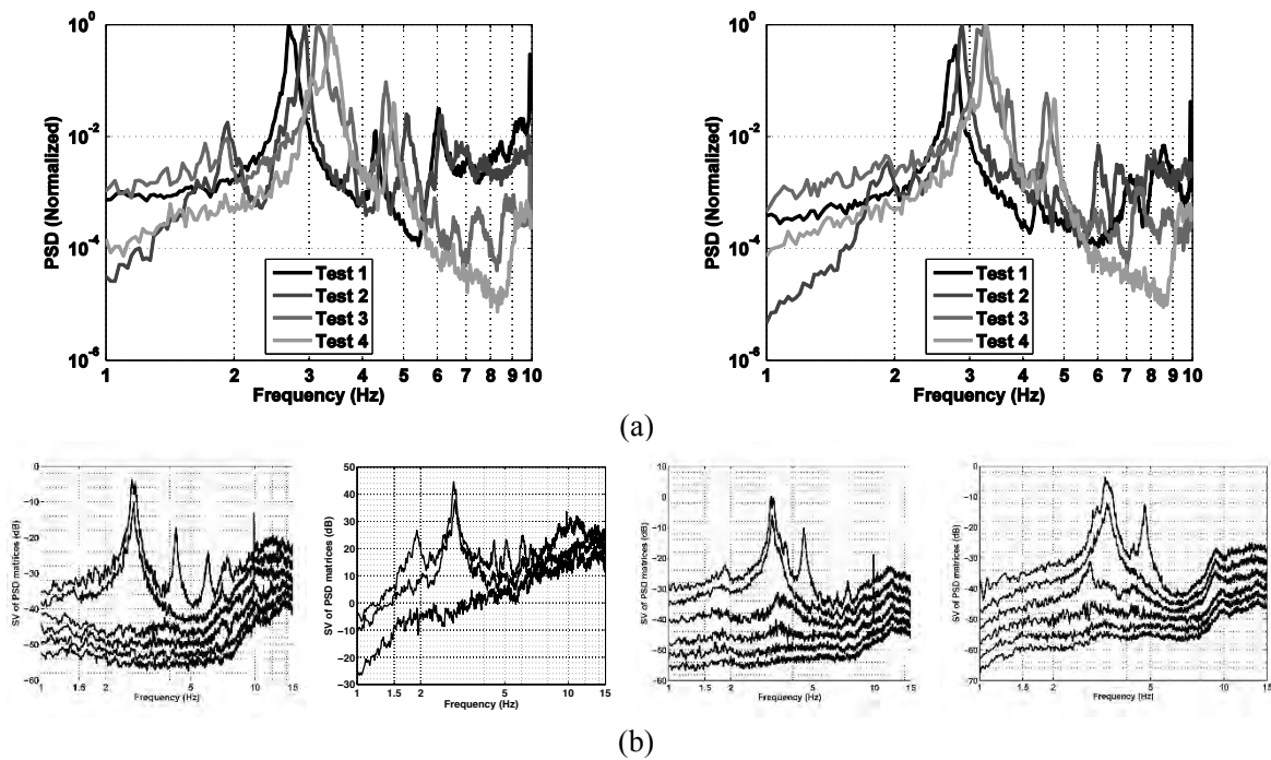
Figure 5. (a) Comparison of the PSD spectra of the 4 tests in the longitudinal and transverse directions and (b) FDD spectra of tests 1, 2, 3 and 4
