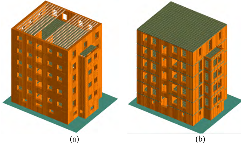
Figure 9. Numerical models for the URM building (a) before and (b) after the retrofit work
