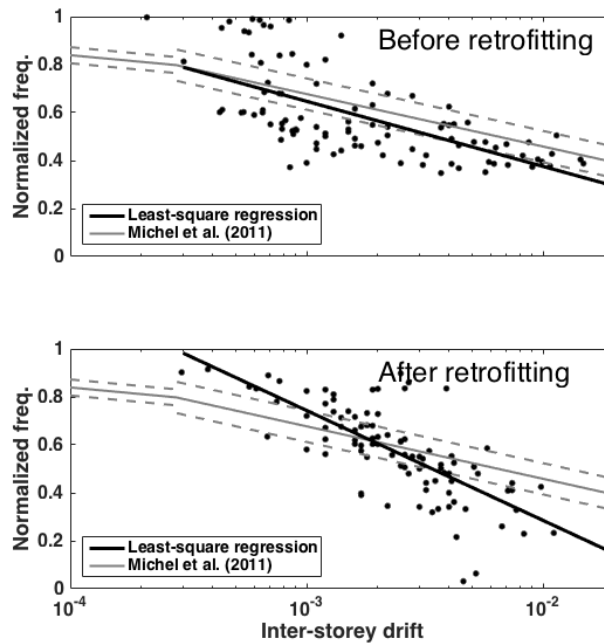
Figure 14. Drop in the modal frequencies (normalized) with the inter-storey drift values
