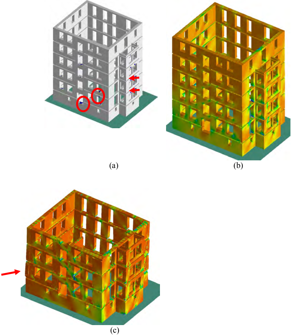
Figure 11. Typical damage mechanisms in the numerical model of the URM building before retrofitting associated to: (a) DG1, (b) DG3 and (c) DG4
