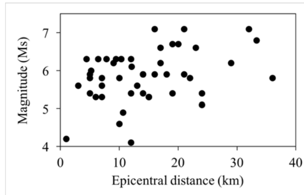
Figure 10. Magnitude-distance distribution of the ground motion records
