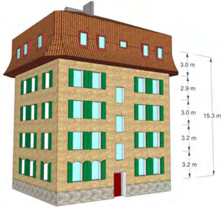
Figure 1. Studied unreinforced masonry residential building.
