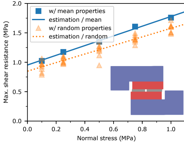
Fig. 6: Comparison of maximum shear resistance with or without considering randomness of material properties of the interface.
