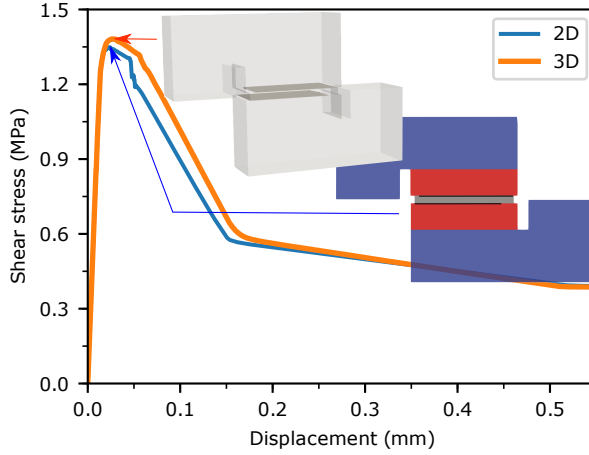
Fig. 5: Comparison of 2D and 3D simulation.
