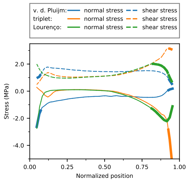
(b) stresses at maximum shear resistance
