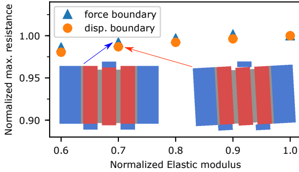
(b) influence of reduced elastic modulus of mortar
