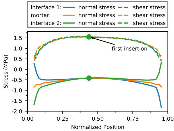
(a) compressive and shear stress at failure initiation
