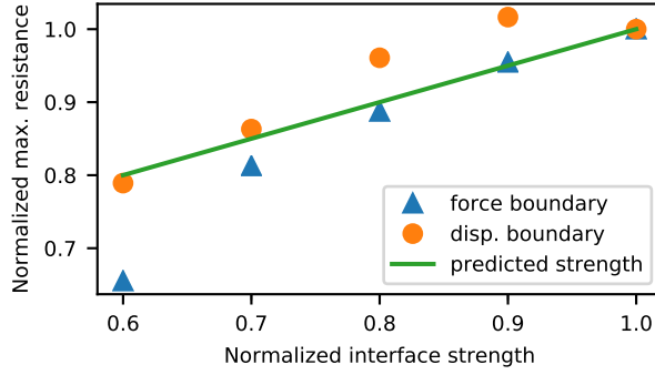
(a) influence of reduced interface strengths
