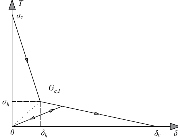
Fig. 2: Traction-separation law.
