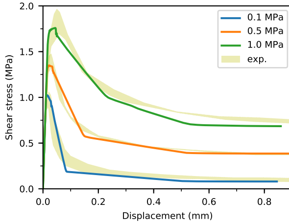
Fig. 4: Calibration of material properties with Van der Pluijm tests.
