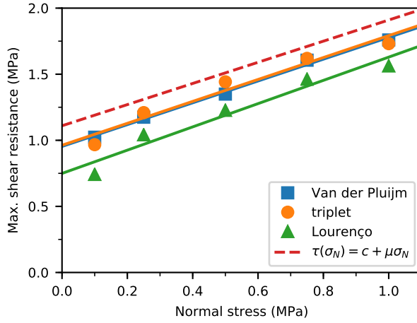
Fig. 7: Maximum shear resistances for different setups w.r.t different normal compression levels.
