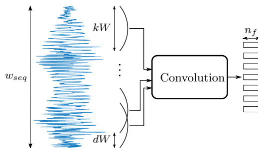
Figure 2: Illustration of first convolution layer processing.
