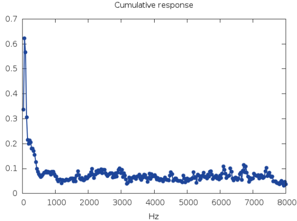
Figure 3: Cumulative frequency response of filters of the first layer.
