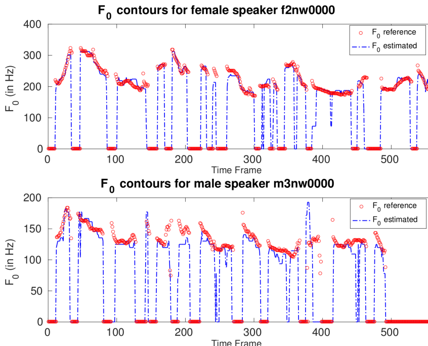
Figure 5: Two examples of the F_0 contours estimated using the first layer filters compared to the reference F_0 from the database.
