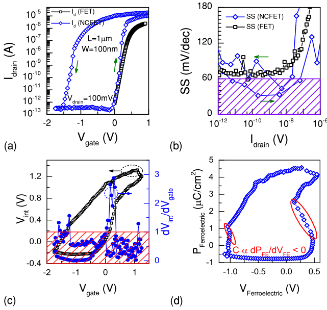
Fig. 4. Transfer characteristic of NCFET-a, where a 20\mu\text{m} \times 20\mu\text{m} PZT capacitor with a thickness of 50\text{nm} is connected to the gate of a commercial n MOSFET (a). Sub-thermal swing (b) is obtained over many decades of current due to the differential voltage amplification of NC. Amplification factor greater than 1 is achieved (c) in the regions corresponding to the negative slope of the ferroelectric polarization (d).
