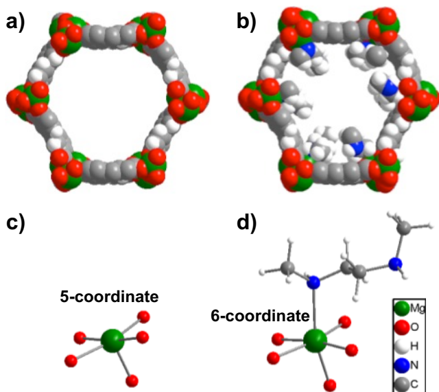
Figure 1. Space-filling models of calculated structures 15 of the activated (a) and mmen-loaded Mg_5(dobpdc) (mmen : Mg = 6 : 6) (b). Ball-and-stick models of the proposed five- (c) and six-coordinate (d) Mg centers.
