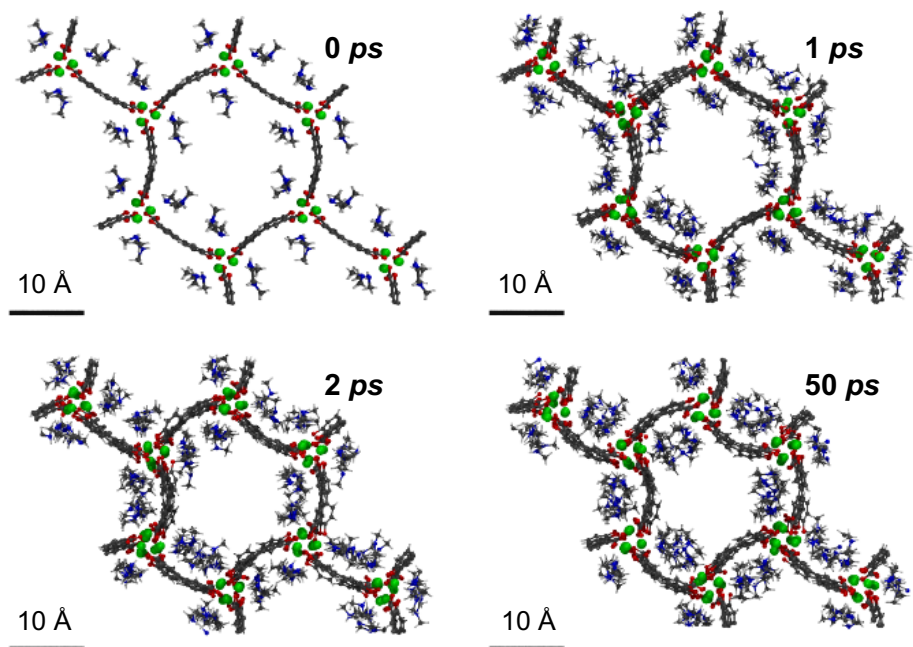
Figure 7. Snapshots of MD simulations for mmen-Mg 2 (dobpdc) (mmen : Mg = 6 : 6) as a function of evolution time. Green, grey, red, blue and white spheres represent Mg, C, O, N and H atoms, respectively.
